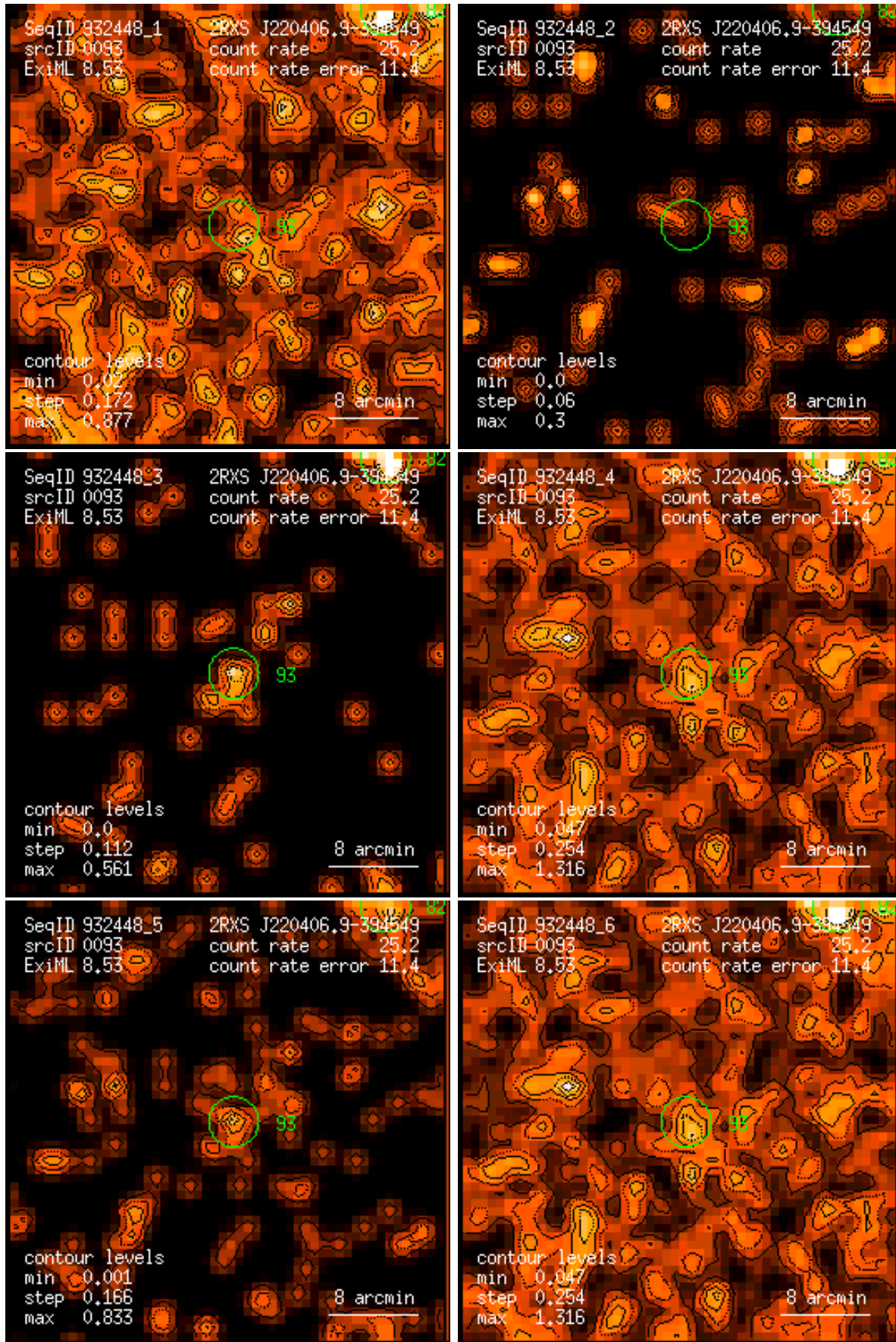
Figure 93: RASS 932448: detection 0093: band rate images, Gaussian filter: (1) PSPC channels 11 – 41, (2) 52 – 90, (3) 91 – 201, (4) 11 – 235, (5) 52 – 201, (6) 11 – 201. Broad band rates in counts/ks. Band rate contour levels in counts/ks/arcmin 2 .
