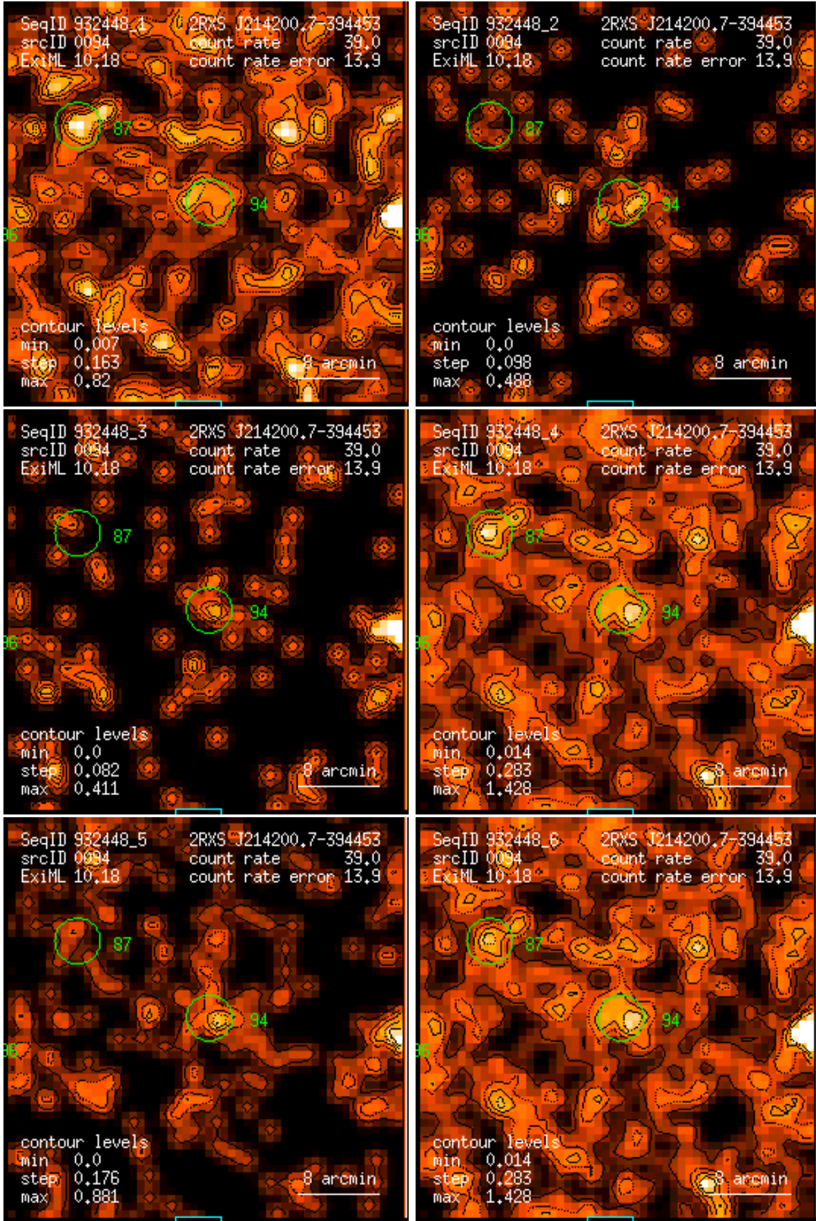
Figure 94: RASS 932448: detection 0094: band rate images, Gaussian filter: (1) PSC channels 11 – 41, (2) 52 – 90, (3) 91 – 201, (4) 11 – 235, (5) 52 – 201, (6) 11 – 201. Broad band rates in counts/ks. Band rate contour levels in counts/ks/arcmin 2 .
