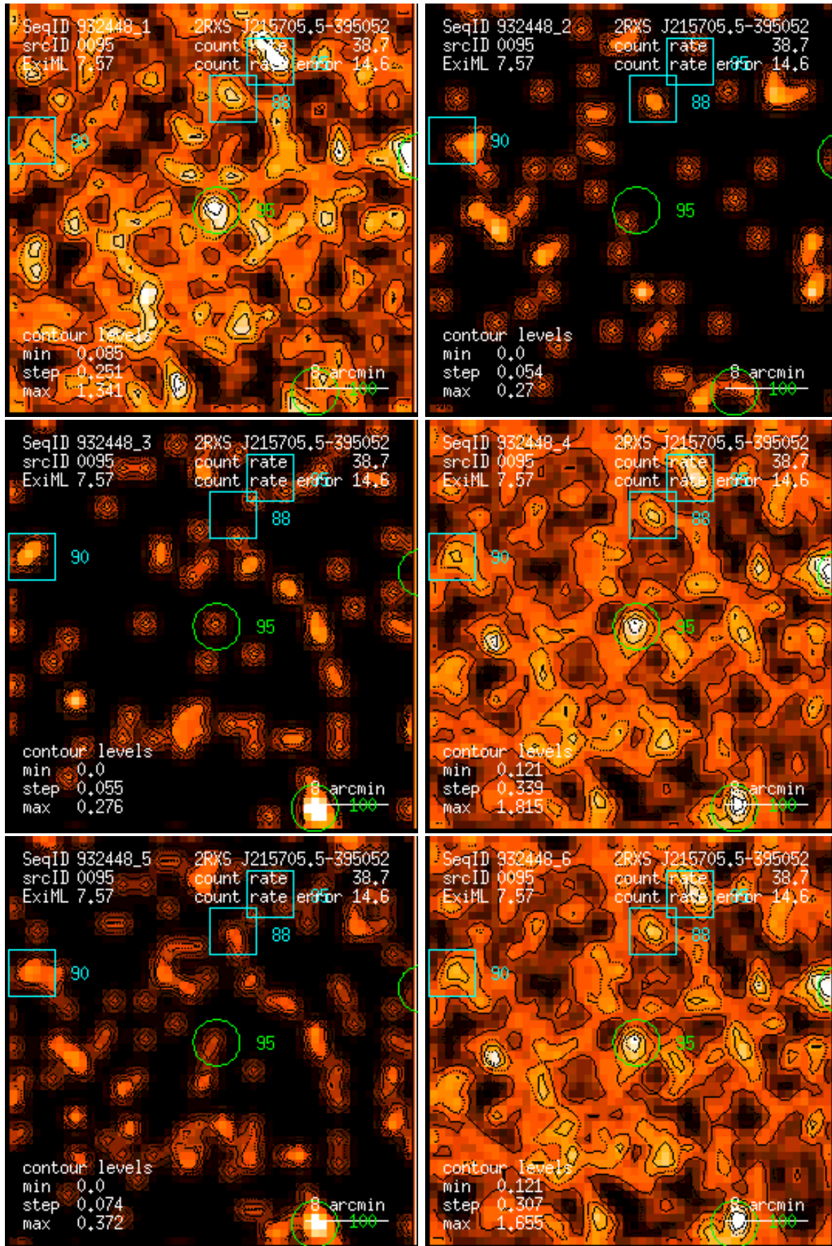
Figure 95: RASS 932448: detection 0095: band rate images, Gaussian filter: (1) PSPC channels 11 – 41, (2) 52 – 90, (3) 91 – 201, (4) 11 – 235, (5) 52 – 201, (6) 11 – 201. Broad band rates in counts/ks. Band rate contour levels in counts/ks/arcmin 2 .
