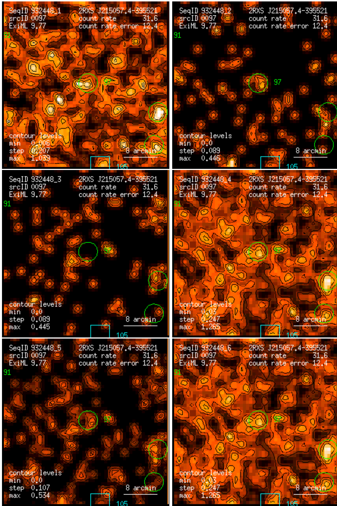
Figure 97: RASS 932448: detection 0097: band rate images, Gaussian filter: (1) PSPC channels 11 – 41, (2) 52 – 90, (3) 91 – 201, (4) 11 – 235, (5) 52 – 201, (6) 11 – 201. Broad band rates in counts/ks. Band rate contour levels in counts/ks/arcmin 2 .
