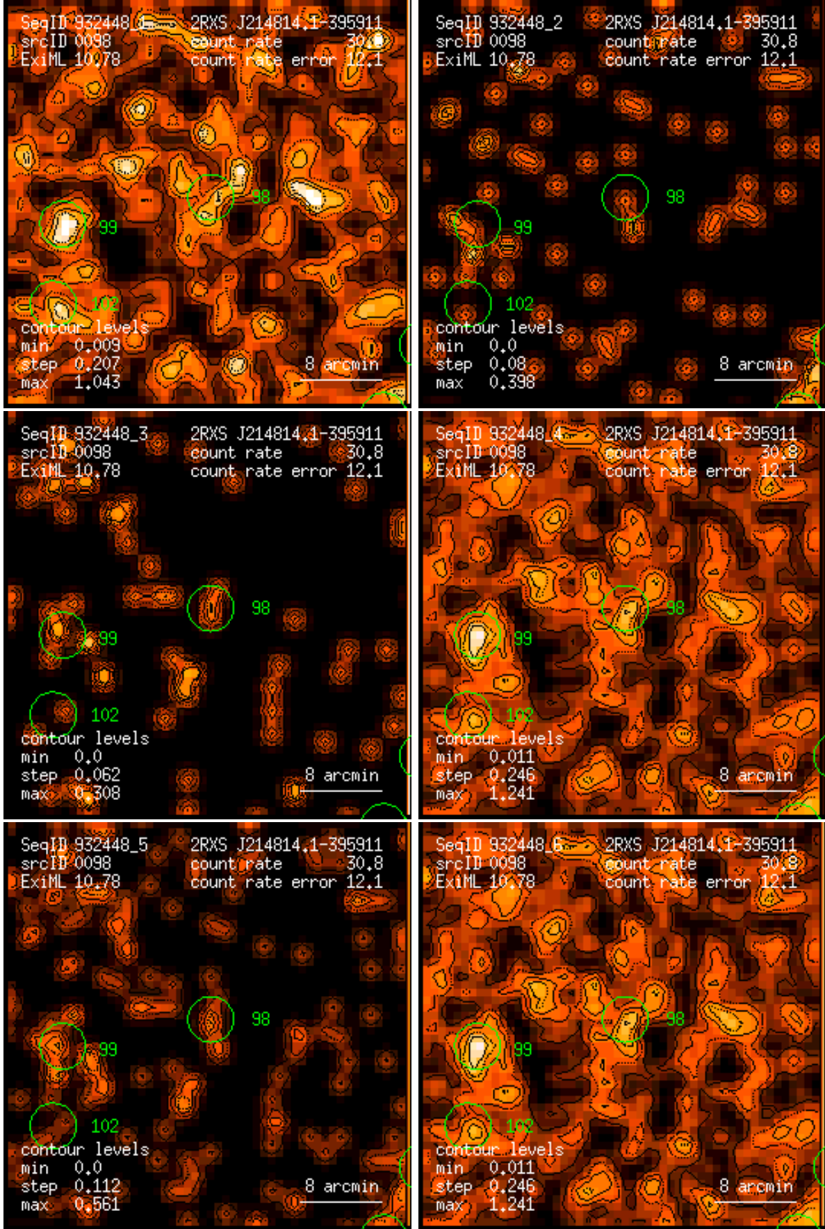
Figure 98: RASS 932448: detection 0098: band rate images, Gaussian filter: (1) PSPC channels 11 – 41, (2) 52 – 90, (3) 91 – 201, (4) 11 – 235, (5) 52 – 201, (6) 11 – 201. Broad band rates in counts/ks. Band rate contour levels in counts/ks/arcmin 2 .
