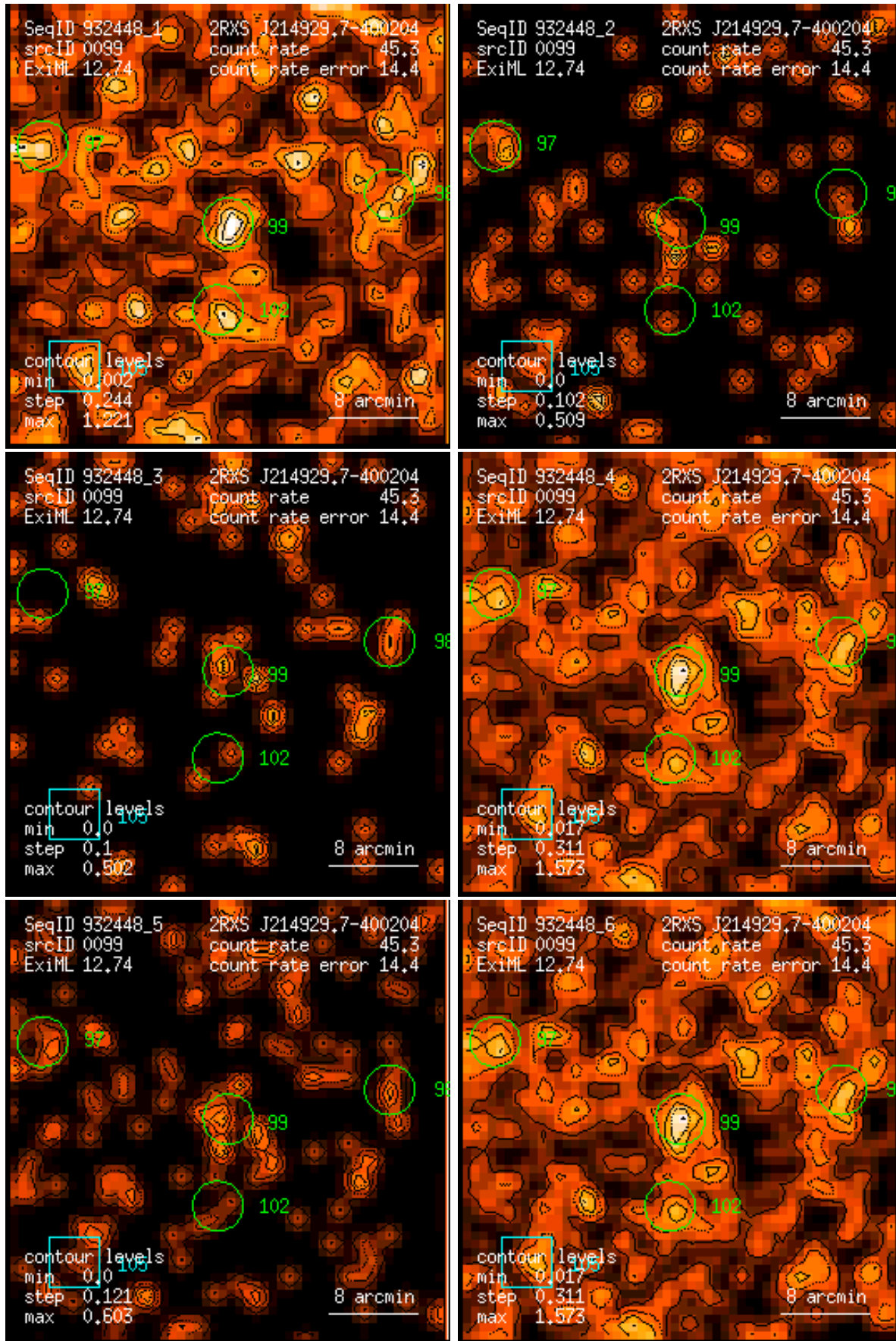
Figure 99: RASS 932448: detection 0099: band rate images, Gaussian filter: (1) PSPC channels 11 – 41, (2) 52 – 90, (3) 91 – 201, (4) 11 – 235, (5) 52 – 201, (6) 11 – 201. Broad band rates in counts/ks. Band rate contour levels in counts/ks/arcmin 2 .
