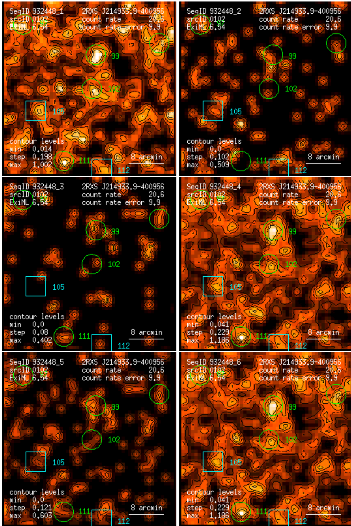
Figure 102: RASS 932448: detection 0102: band rate images, Gaussian filter: (1) PSPC channels 11 – 41, (2) 52 – 90, (3) 91 – 201, (4) 11 – 235, (5) 52 – 201, (6) 11 – 201. Broad band rates in counts/ks. Band rate contour levels in counts/ks/arcmin 2 .
