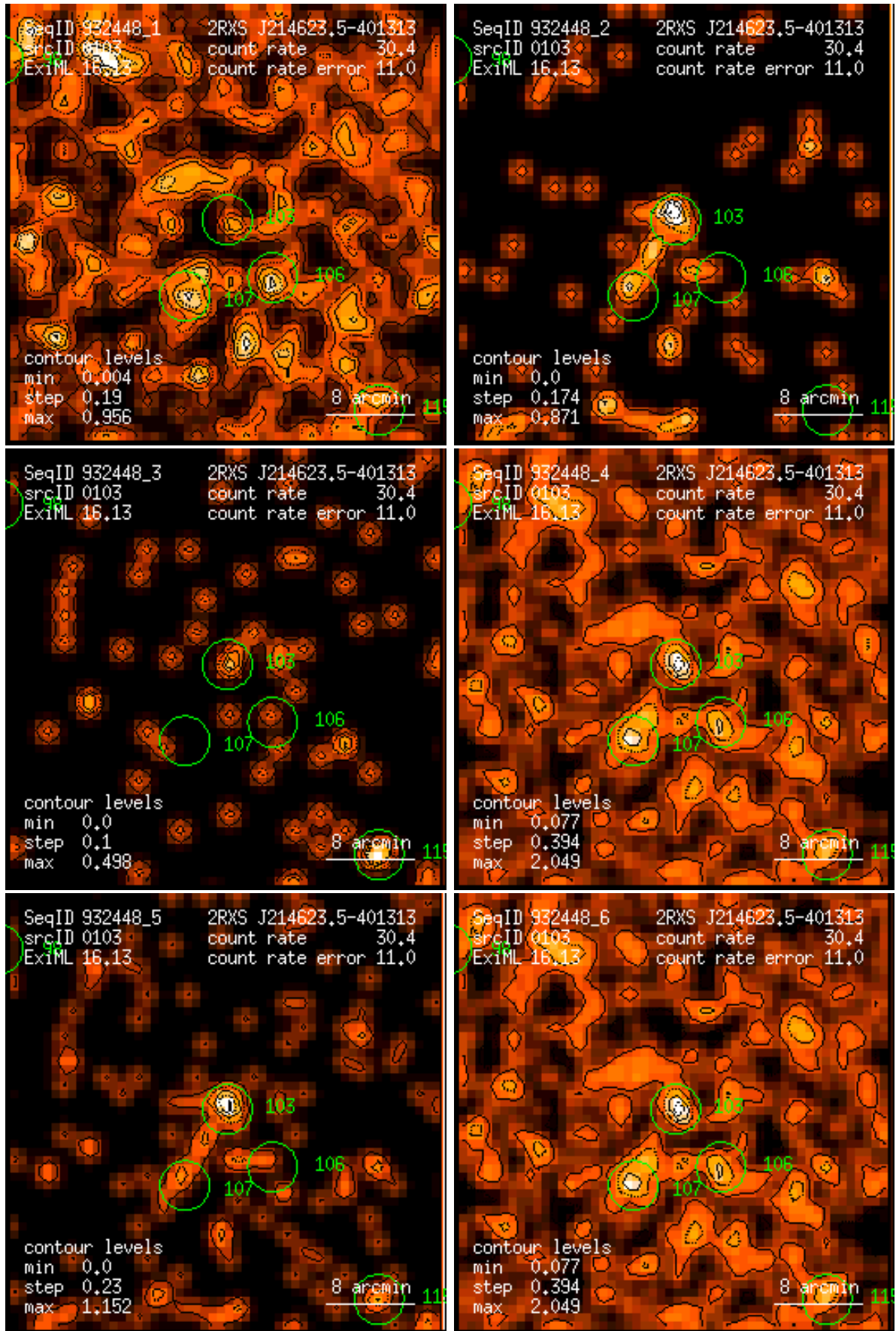
Figure 103: RASS 932448: detection 0103: band rate images, Gaussian filter: (1) PSPC channels 11 – 41, (2) 52 – 90, (3) 91 – 201, (4) 11 – 235, (5) 52 – 201, (6) 11 – 201. Broad band rates in counts/ks. Band rate contour levels in counts/ks/arcmin 2 .
