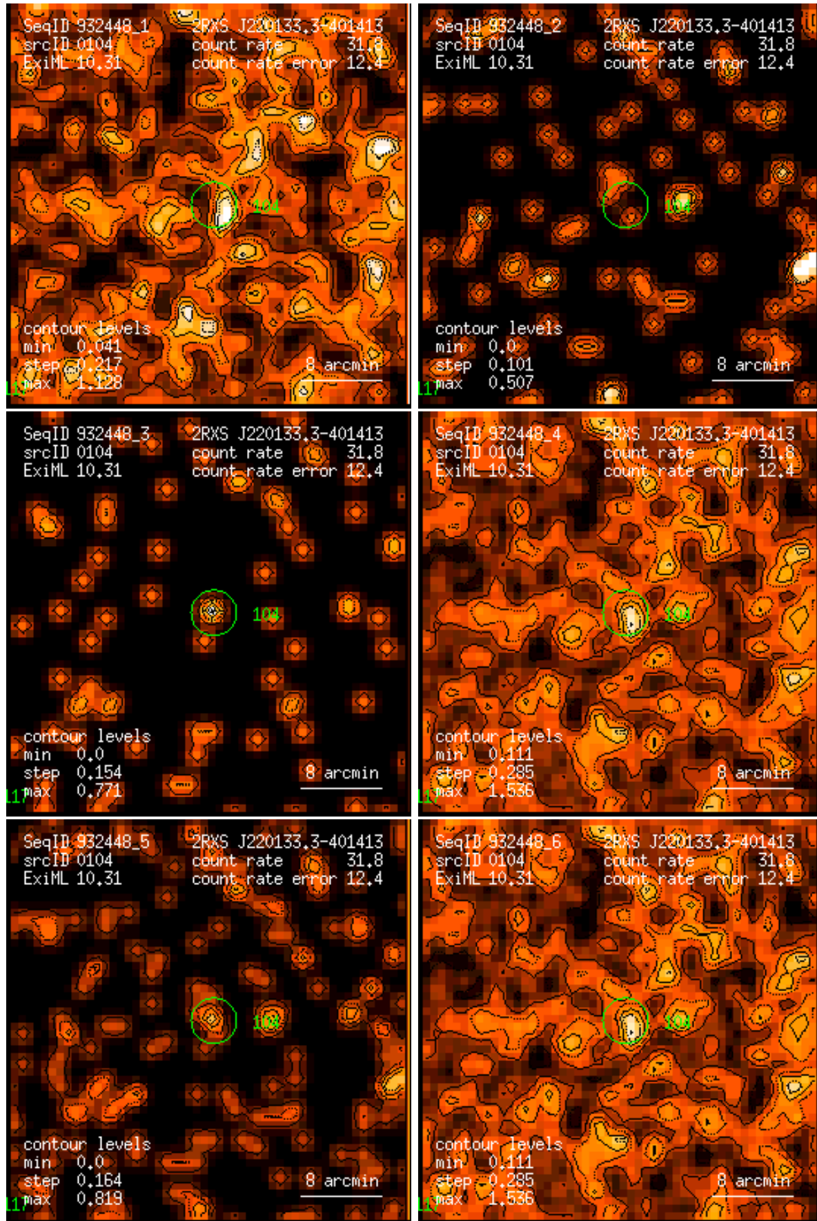
Figure 104: RASS 932448: detection 0104: band rate images, Gaussian filter: (1) PSPC channels 11 – 41, (2) 52 – 90, (3) 91 – 201, (4) 11 – 235, (5) 52 – 201, (6) 11 – 201. Broad band rates in counts/ks. Band rate contour levels in counts/ks/arcmin 2 .
