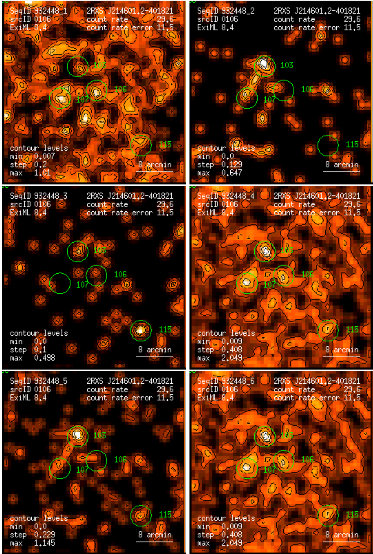
Figure 106: RASS 932448: detection 0106: band rate images, Gaussian filter: (1) PSPC channels 11 – 41, (2) 52 – 90, (3) 91 – 201, (4) 11 – 235, (5) 52 – 201, (6) 11 – 201. Broad band rates in counts/ks. Band rate contour levels in counts/ks/arcmin 2 .
