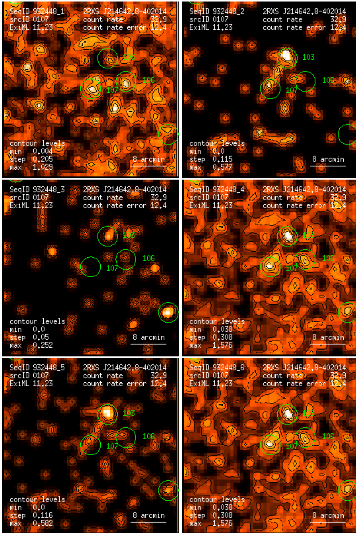
Figure 107: RASS 932448: detection 0107: band rate images, Gaussian filter: (1) PSPC channels 11 – 41, (2) 52 – 90, (3) 91 – 201, (4) 11 – 235, (5) 52 – 201, (6) 11 – 201. Broad band rates in counts/ks. Band rate contour levels in counts/ks/arcmin 2 .
