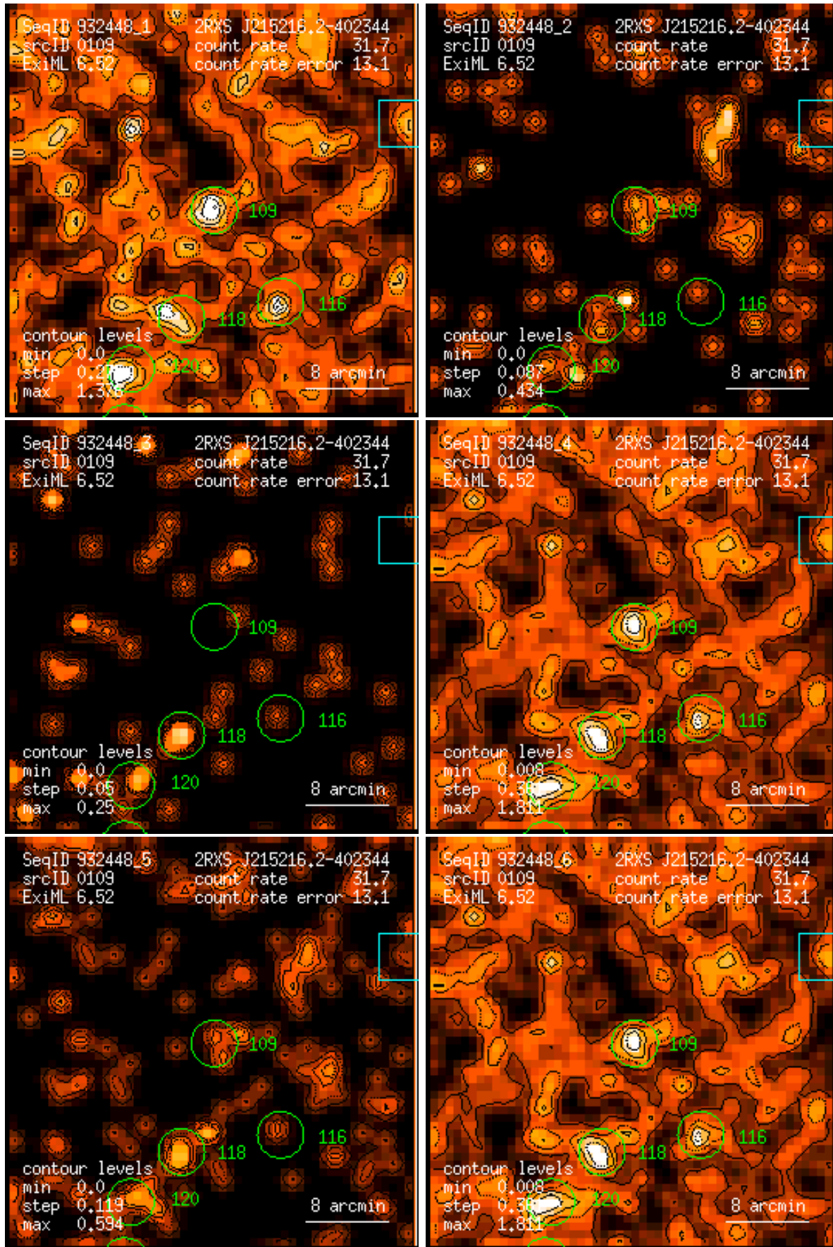
Figure 109: RASS 932448: detection 0109: band rate images, Gaussian filter: (1) PSPC channels 11 – 41, (2) 52 – 90, (3) 91 – 201, (4) 11 – 235, (5) 52 – 201, (6) 11 – 201. Broad band rates in counts/ks. Band rate contour levels in counts/ks/arcmin 2 .
