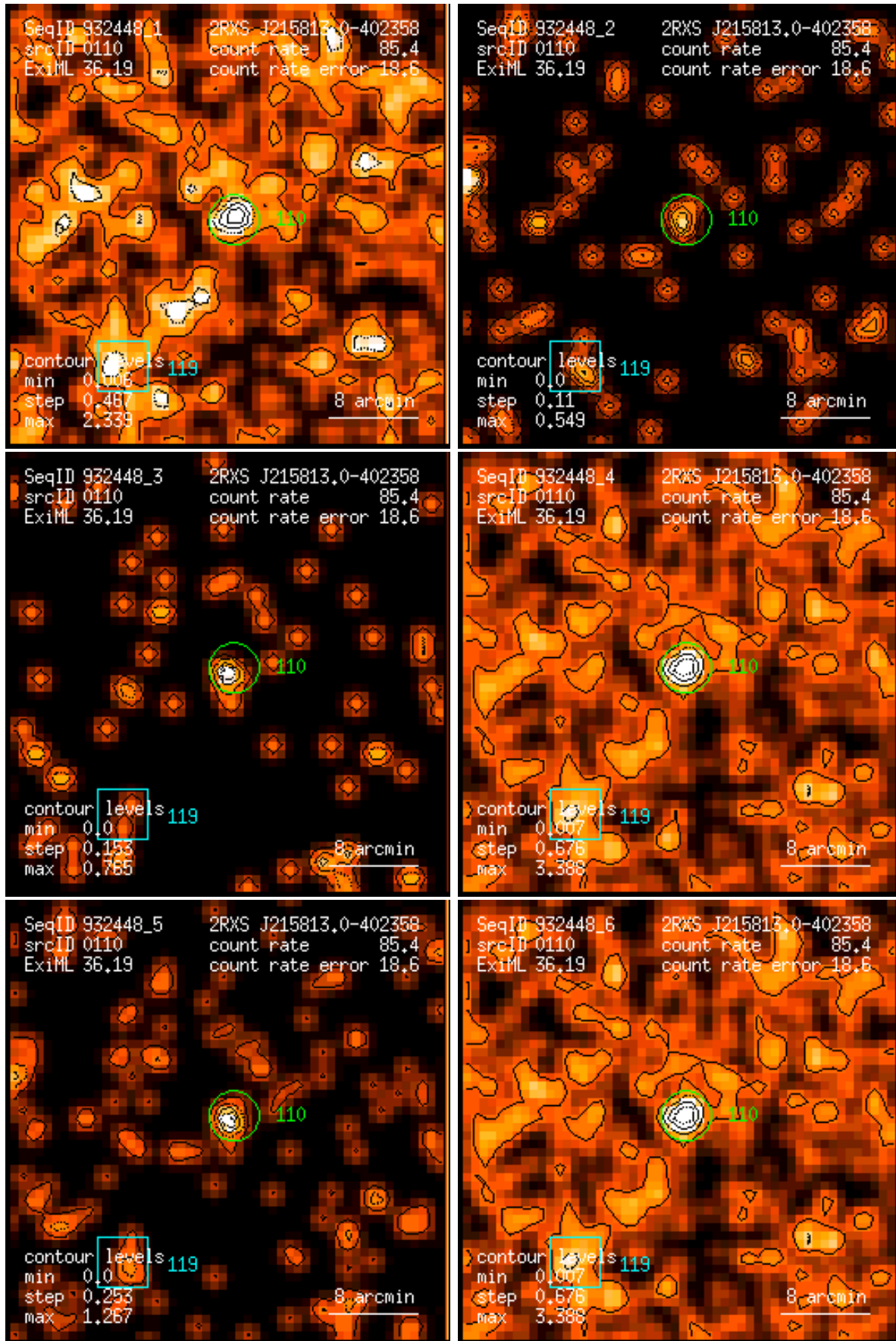
Figure 110: RASS 932448: detection 0110: band rate images, Gaussian filter: (1) PSPC channels 11 – 41, (2) 52 – 90, (3) 91 – 201, (4) 11 – 235, (5) 52 – 201, (6) 11 – 201. Broad band rates in counts/ks. Band rate contour levels in counts/ks/arcmin 2 .
