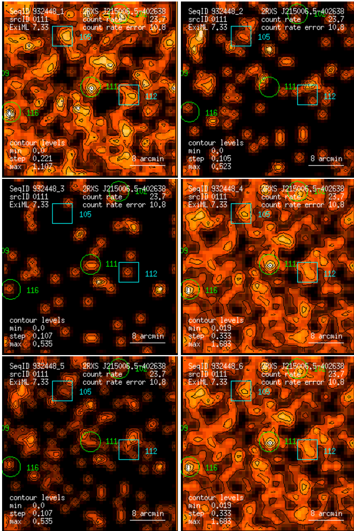
Figure 111: RASS 932448: detection 0111: band rate images, Gaussian filter: (1) PSPC channels 11 – 41, (2) 52 – 90, (3) 91 – 201, (4) 11 – 235, (5) 52 – 201, (6) 11 – 201. Broad band rates in counts/ks. Band rate contour levels in counts/ks/arcmin 2 .
