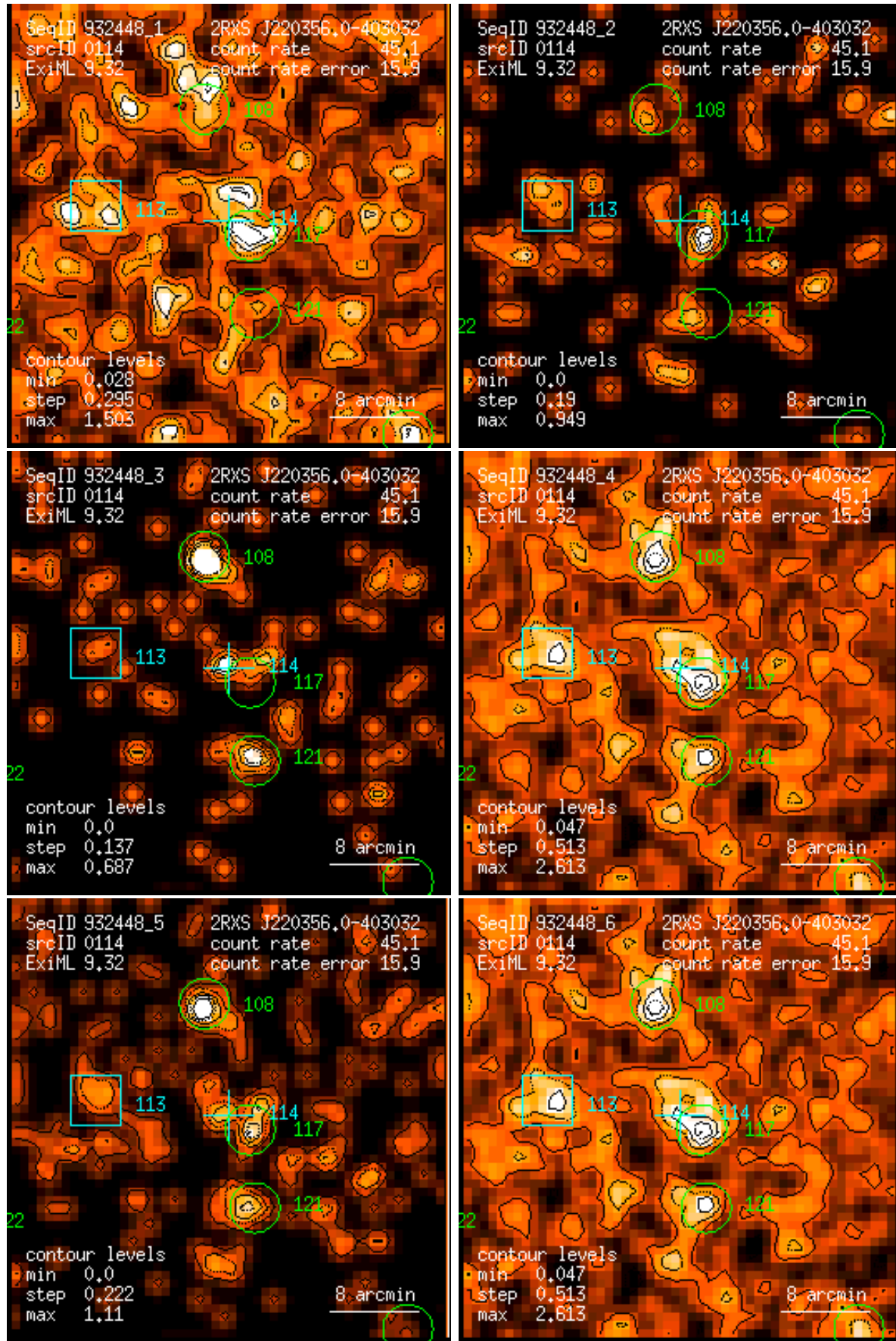
Figure 114: RASS 932448: detection 0114: band rate images, Gaussian filter: (1) PSPC channels 11 – 41, (2) 52 – 90, (3) 91 – 201, (4) 11 – 235, (5) 52 – 201, (6) 11 – 201. Broad band rates in counts/ks. Band rate contour levels in counts/ks/arcmin 2 .
