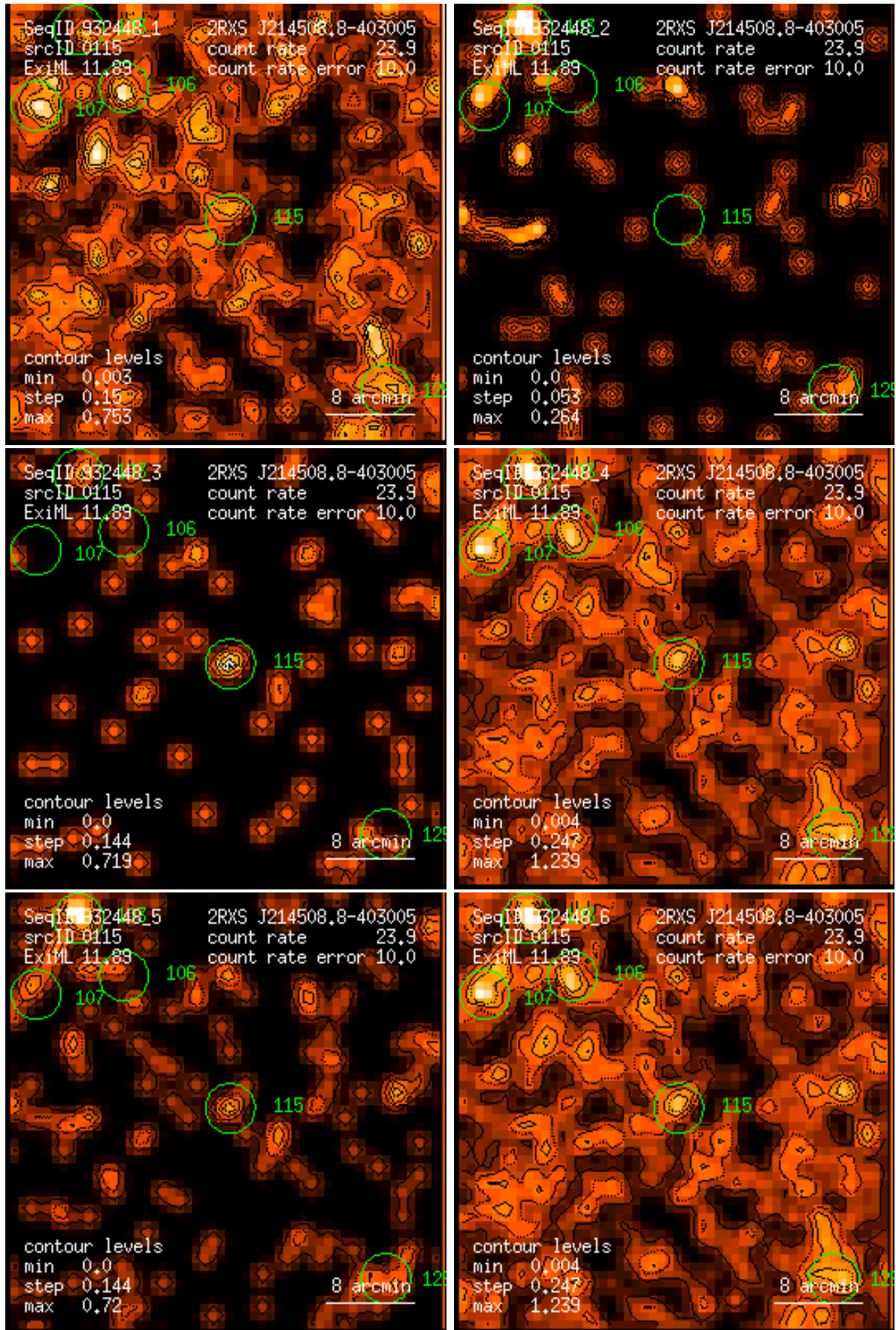
Figure 115: RASS 932448: detection 0115: band rate images, Gaussian filter: (1) PSPC channels 11 – 41, (2) 52 – 90, (3) 91 – 201, (4) 11 – 235, (5) 52 – 201, (6) 11 – 201. Broad band rates in counts/ks. Band rate contour levels in counts/ks/arcmin 2 .
