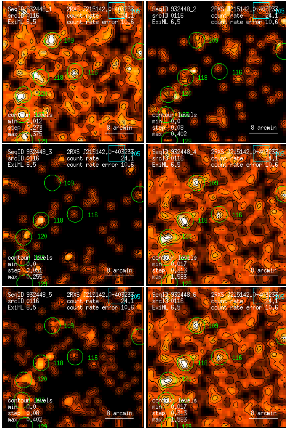
Figure 116: RASS 932448: detection 0116: band rate images, Gaussian filter: (1) PSPC channels 11 – 41, (2) 52 – 90, (3) 91 – 201, (4) 11 – 235, (5) 52 – 201, (6) 11 – 201. Broad band rates in counts/ks. Band rate contour levels in counts/ks/arcmin 2 .
