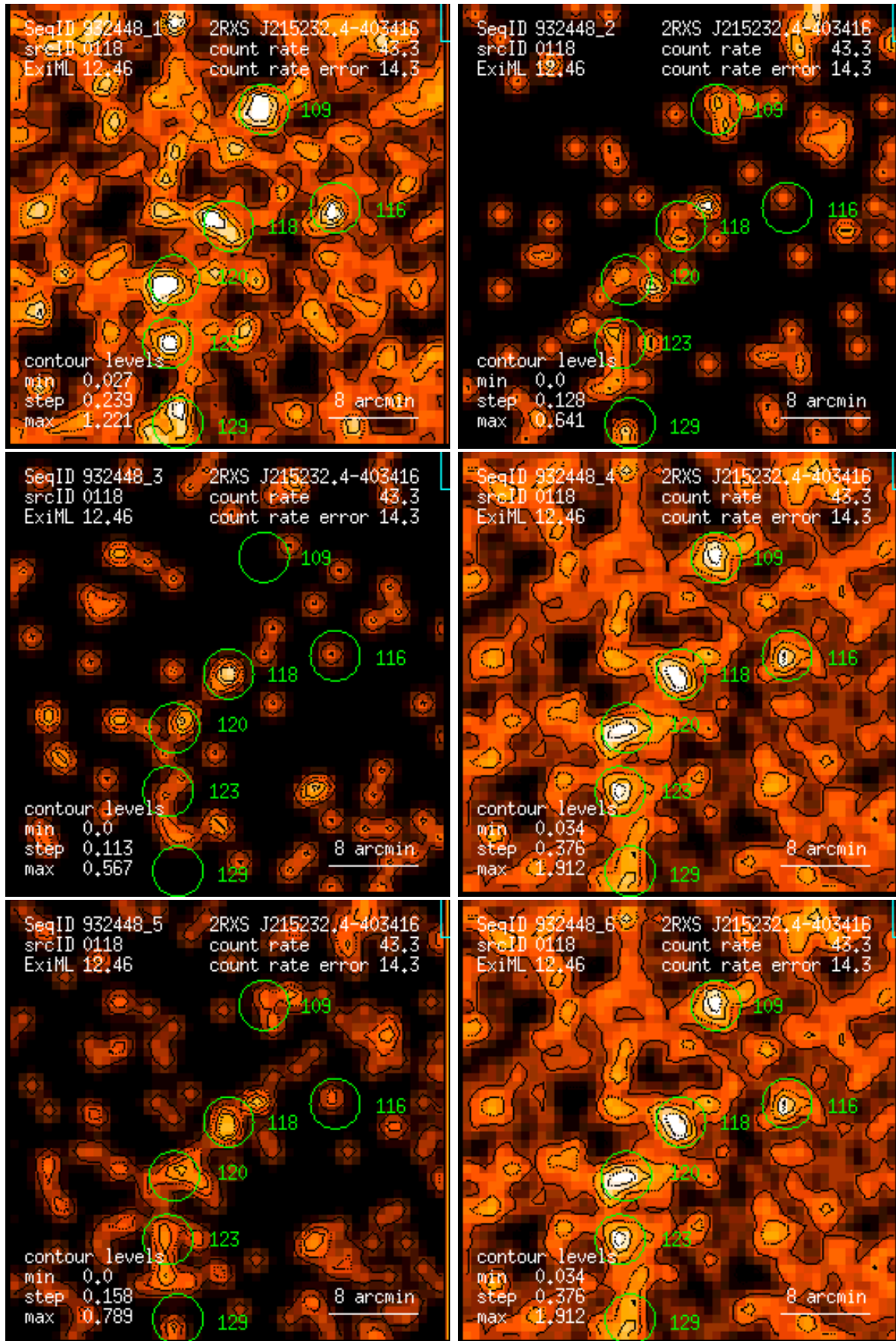
Figure 118: RASS 932448: detection 0118: band rate images, Gaussian filter: (1) PSPC channels 11 – 41, (2) 52 – 90, (3) 91 – 201, (4) 11 – 235, (5) 52 – 201, (6) 11 – 201. Broad band rates in counts/ks. Band rate contour levels in counts/ks/arcmin 2 .
