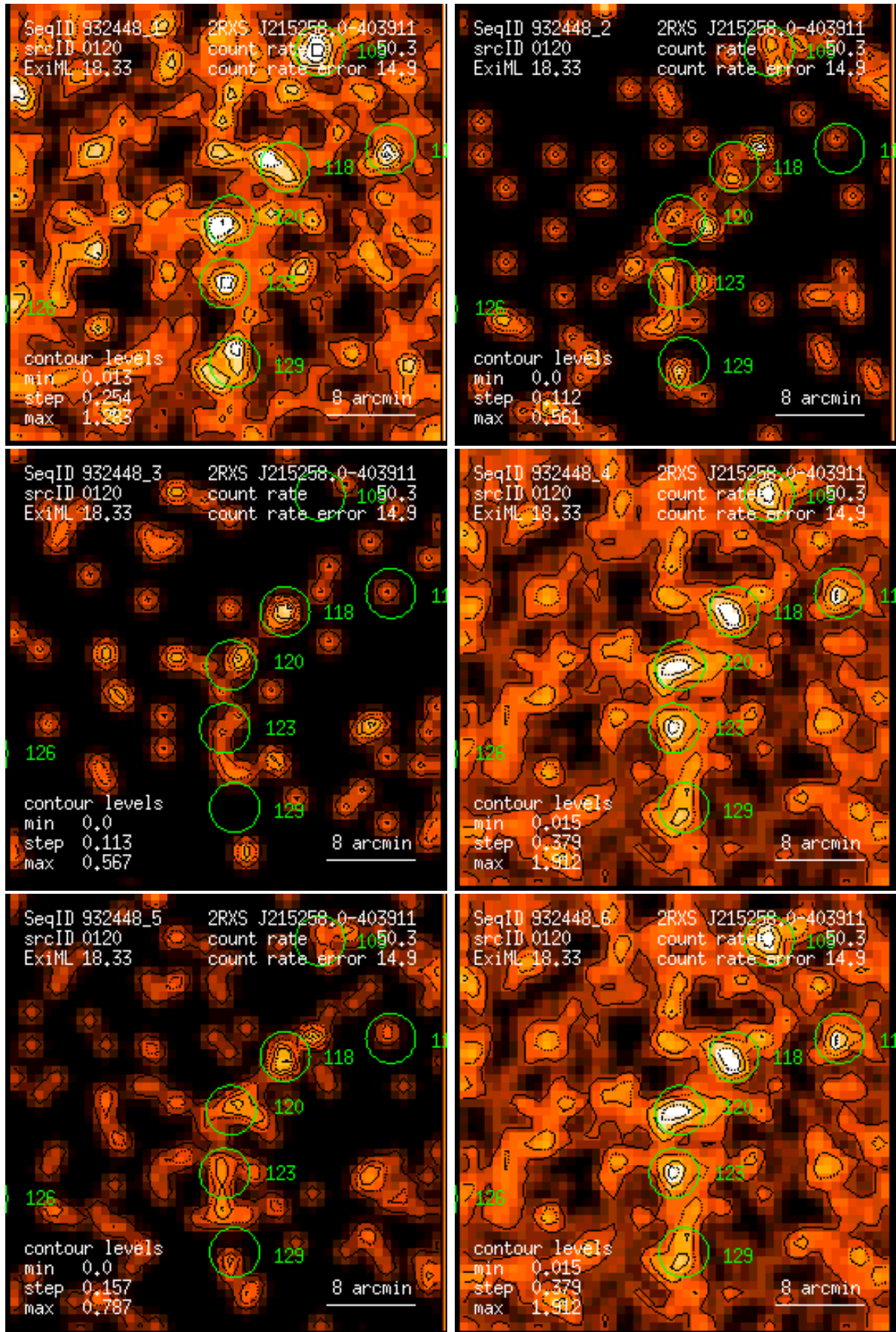
Figure 120: RASS 932448: detection 0120: band rate images, Gaussian filter: (1) PSPC channels 11 – 41, (2) 52 – 90, (3) 91 – 201, (4) 11 – 235, (5) 52 – 201, (6) 11 – 201. Broad band rates in counts/ks. Band rate contour levels in counts/ks/arcmin 2 .
