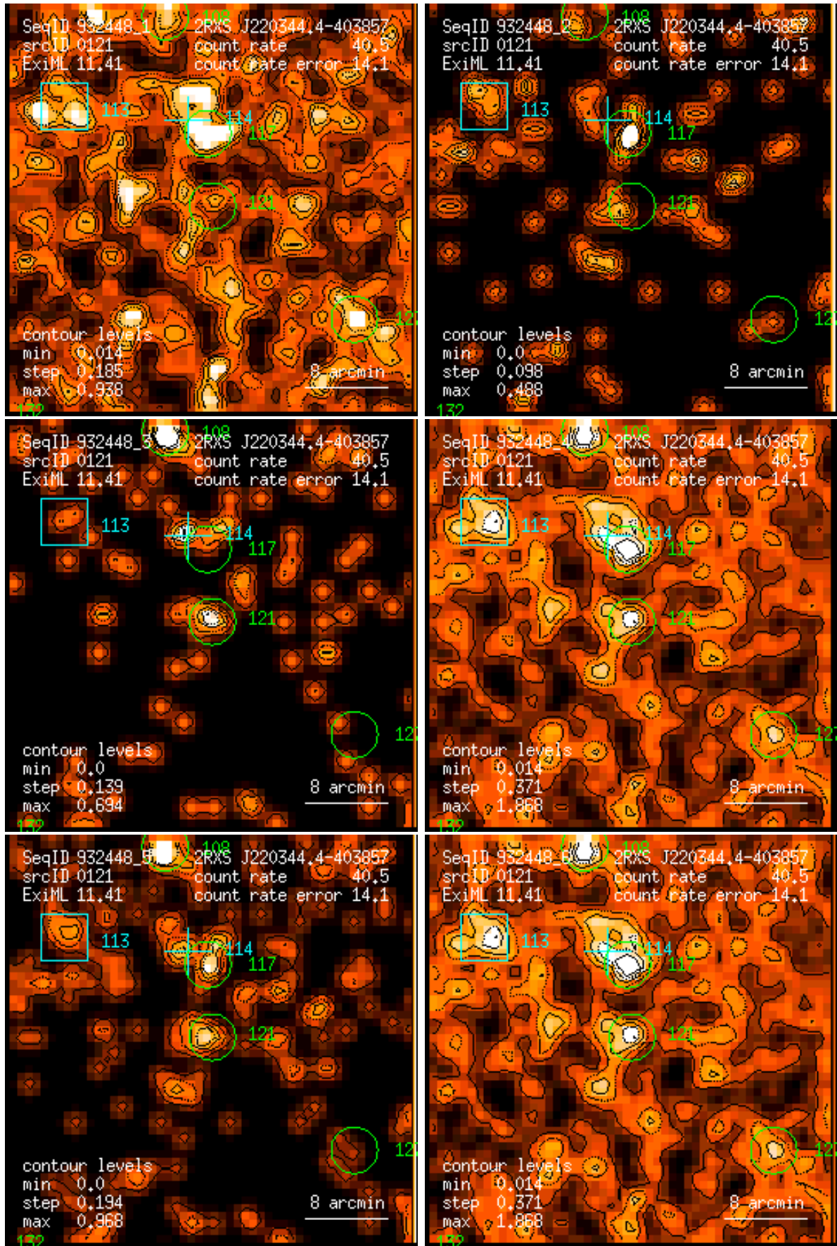
Figure 121: RASS 932448: detection 0121: band rate images, Gaussian filter: (1) PSPC channels 11 – 41, (2) 52 – 90, (3) 91 – 201, (4) 11 – 235, (5) 52 – 201, (6) 11 – 201. Broad band rates in counts/ks. Band rate contour levels in counts/ks/arcmin 2 .
