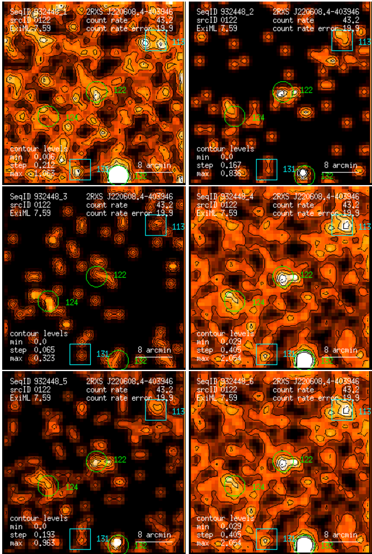
Figure 122: RASS 932448: detection 0122: band rate images, Gaussian filter: (1) PSPC channels 11 – 41, (2) 52 – 90, (3) 91 – 201, (4) 11 – 235, (5) 52 – 201, (6) 11 – 201. Broad band rates in counts/ks. Band rate contour levels in counts/ks/arcmin 2 .
