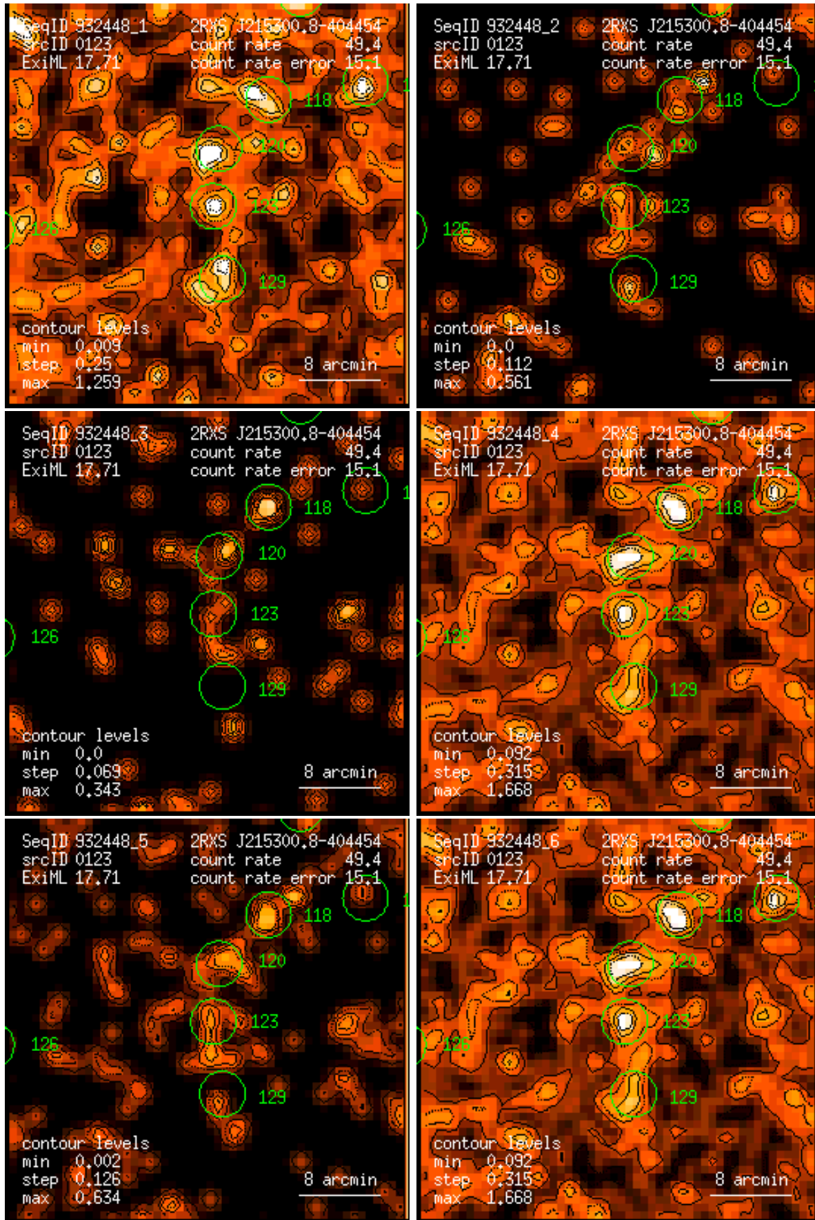
Figure 123: RASS 932448: detection 0123: band rate images, Gaussian filter: (1) PSPC channels 11 – 41, (2) 52 – 90, (3) 91 – 201, (4) 11 – 235, (5) 52 – 201, (6) 11 – 201. Broad band rates in counts/ks. Band rate contour levels in counts/ks/arcmin 2 .
