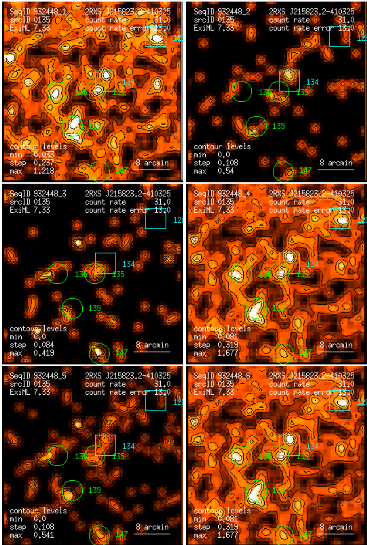
Figure 135: RASS 932448: detection 0135: band rate images, Gaussian filter: (1) PSPC channels 11 – 41, (2) 52 – 90, (3) 91 – 201, (4) 11 – 235, (5) 52 – 201, (6) 11 – 201. Broad band rates in counts/ks. Band rate contour levels in counts/ks/arcmin 2 .
