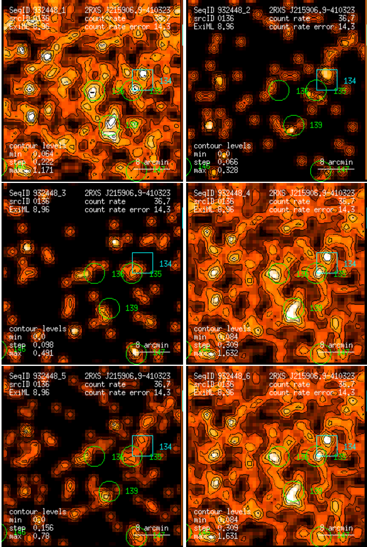
Figure 136: RASS 932448: detection 0136: band rate images, Gaussian filter: (1) PSPC channels 11 – 41, (2) 52 – 90, (3) 91 – 201, (4) 11 – 235, (5) 52 – 201, (6) 11 – 201. Broad band rates in counts/ks. Band rate contour levels in counts/ks/arcmin 2 .
