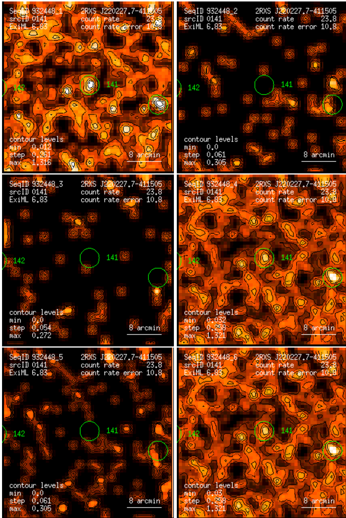
Figure 141: RASS 932448: detection 0141: band rate images, Gaussian filter: (1) PSPC channels 11 – 41, (2) 52 – 90, (3) 91 – 201, (4) 11 – 235, (5) 52 – 201, (6) 11 – 201. Broad band rates in counts/ks. Band rate contour levels in counts/ks/arcmin 2 .
