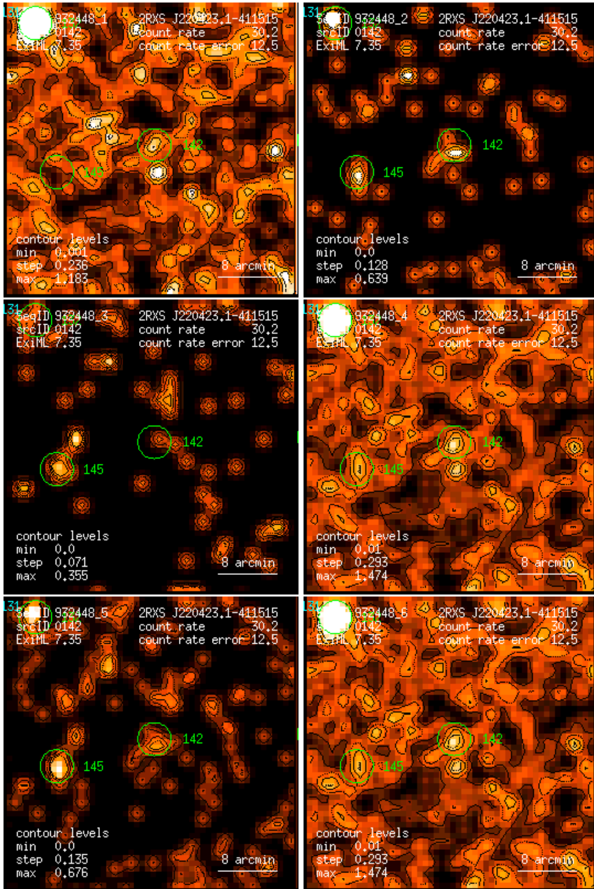
Figure 142: RASS 932448: detection 0142: band rate images, Gaussian filter: (1) PSPC channels 11 – 41, (2) 52 – 90, (3) 91 – 201, (4) 11 – 235, (5) 52 – 201, (6) 11 – 201. Broad band rates in counts/ks. Band rate contour levels in counts/ks/arcmin 2 .
