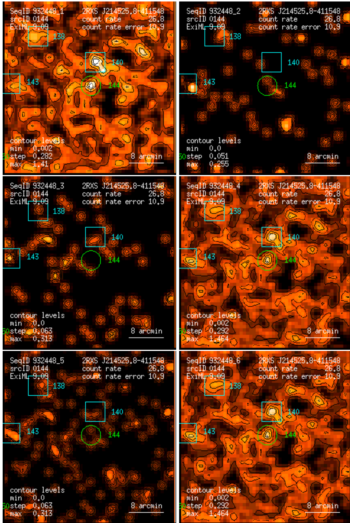
Figure 144: RASS 932448: detection 0144: band rate images, Gaussian filter: (1) PSPC channels 11 – 41, (2) 52 – 90, (3) 91 – 201, (4) 11 – 235, (5) 52 – 201, (6) 11 – 201. Broad band rates in counts/ks. Band rate contour levels in counts/ks/arcmin 2 .
