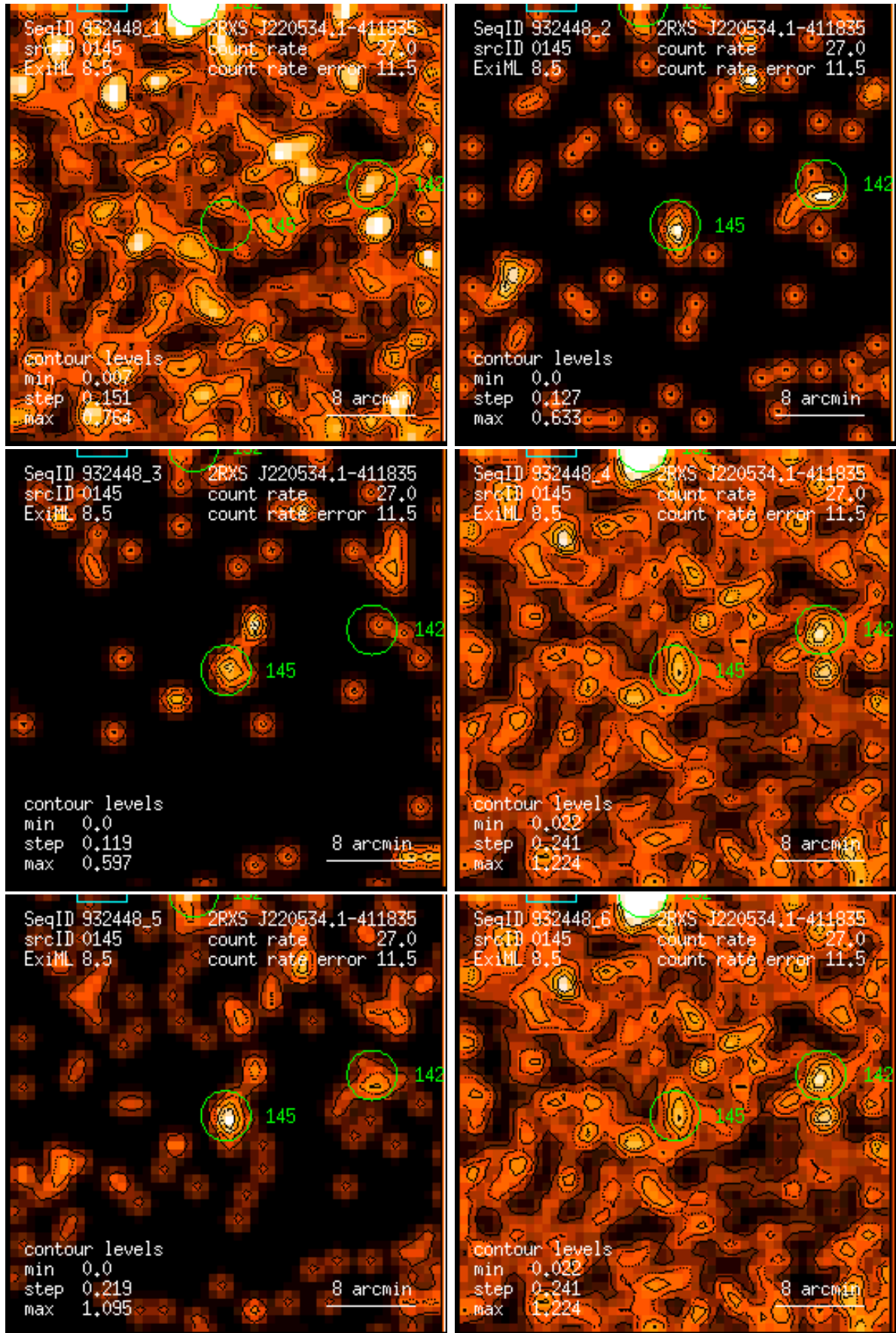
Figure 145: RASS 932448: detection 0145: band rate images, Gaussian filter: (1) PSPC channels 11 – 41, (2) 52 – 90, (3) 91 – 201, (4) 11 – 235, (5) 52 – 201, (6) 11 – 201. Broad band rates in counts/ks. Band rate contour levels in counts/ks/arcmin 2 .
