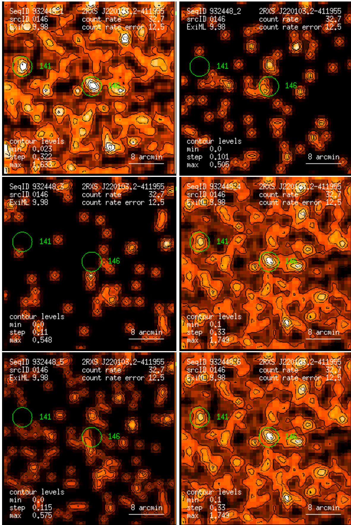
Figure 146: RASS 932448: detection 0146: band rate images, Gaussian filter: (1) PSPC channels 11 – 41, (2) 52 – 90, (3) 91 – 201, (4) 11 – 235, (5) 52 – 201, (6) 11 – 201. Broad band rates in counts/ks. Band rate contour levels in counts/ks/arcmin 2 .
