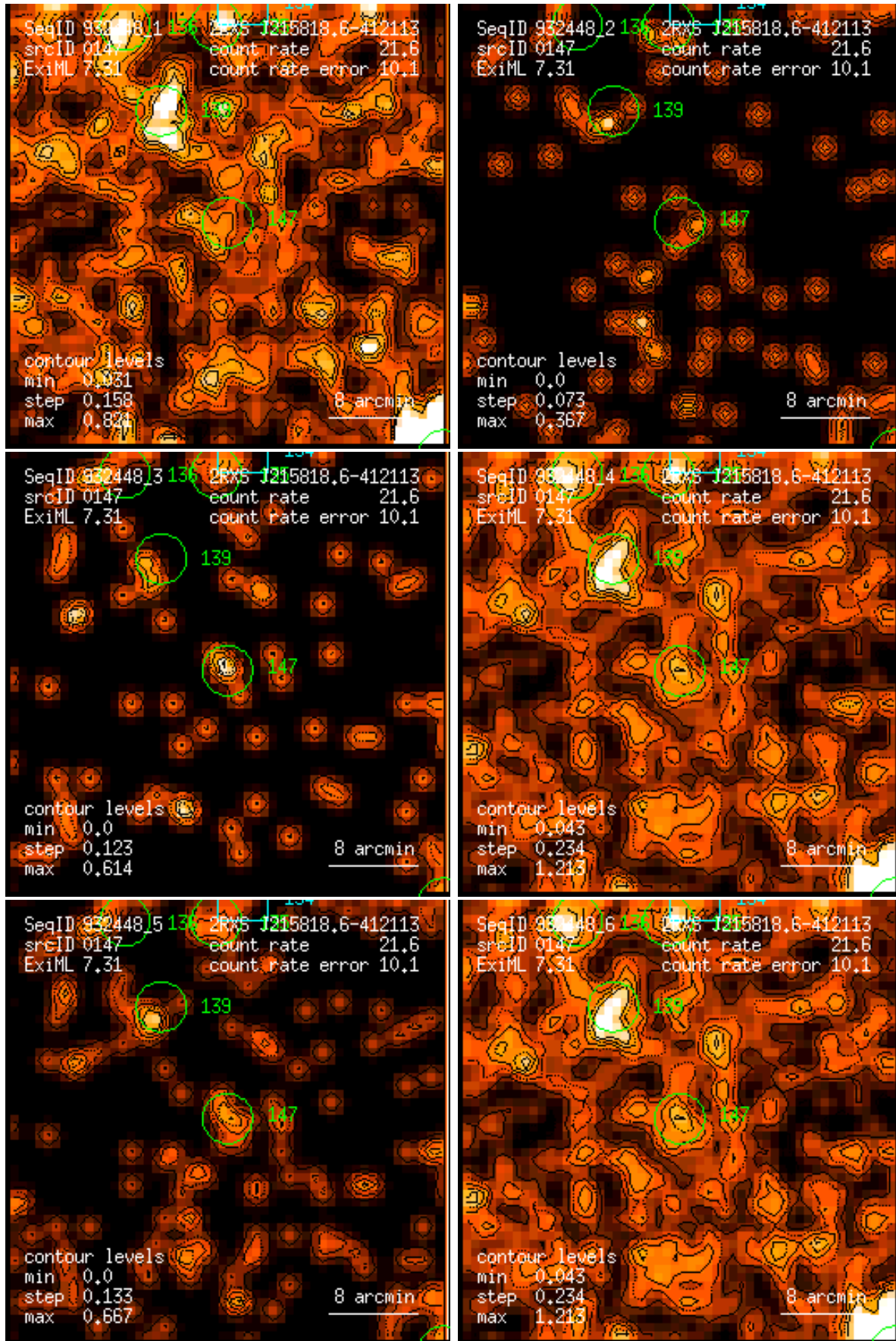
Figure 147: RASS 932448: detection 0147: band rate images, Gaussian filter: (1) PSPC channels 11 – 41, (2) 52 – 90, (3) 91 – 201, (4) 11 – 235, (5) 52 – 201, (6) 11 – 201. Broad band rates in counts/ks. Band rate contour levels in counts/ks/arcmin 2 .
