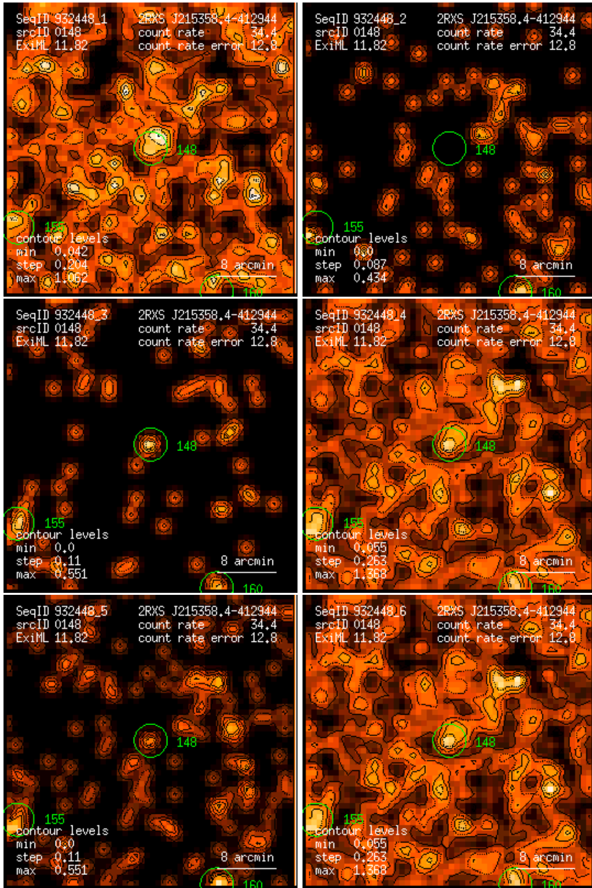
Figure 148: RASS 932448: detection 0148: band rate images, Gaussian filter: (1) PSPC channels 11 – 41, (2) 52 – 90, (3) 91 – 201, (4) 11 – 235, (5) 52 – 201, (6) 11 – 201. Broad band rates in counts/ks. Band rate contour levels in counts/ks/arcmin 2 .
