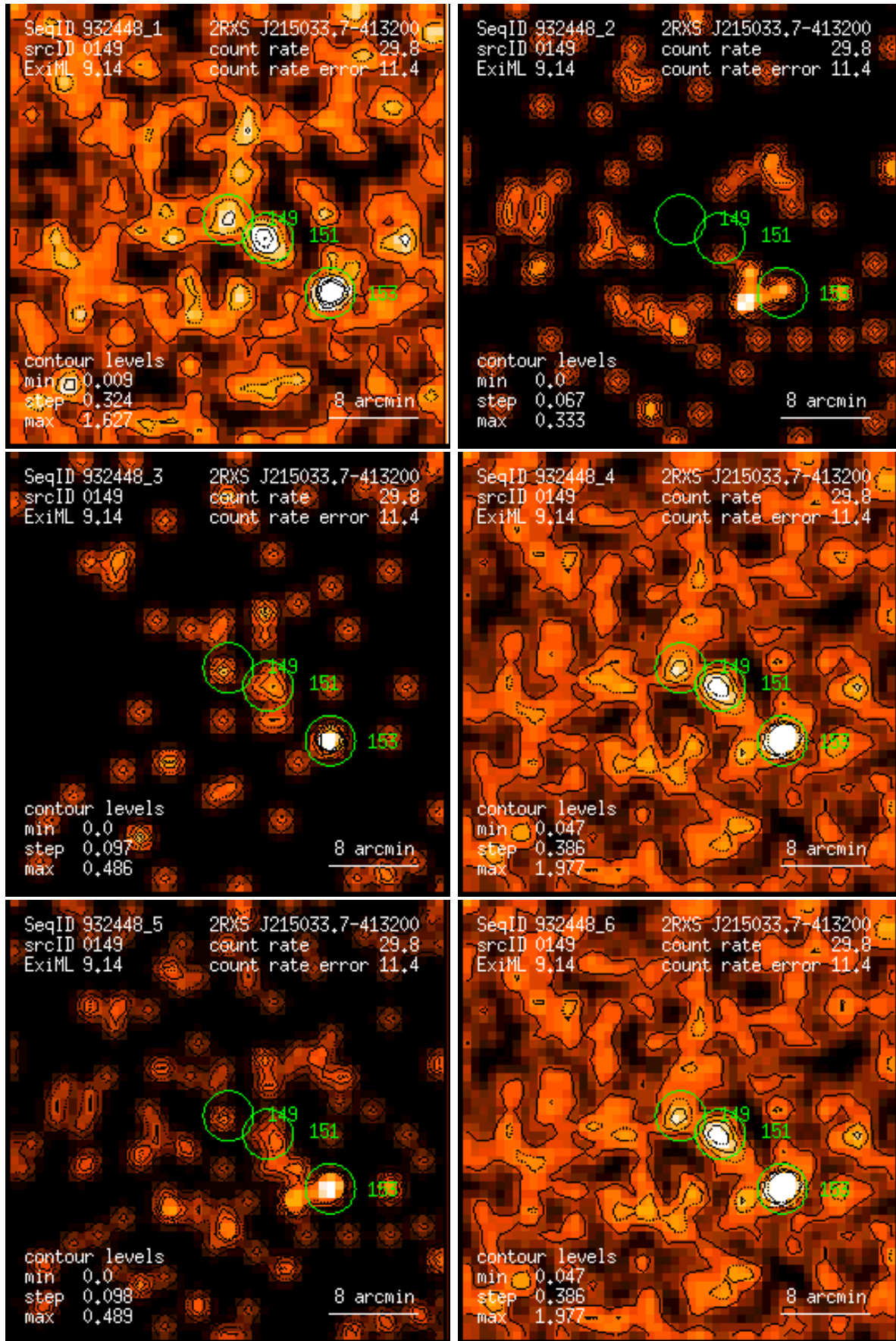
Figure 149: RASS 932448: detection 0149: band rate images, Gaussian filter: (1) PSPC channels 11 – 41, (2) 52 – 90, (3) 91 – 201, (4) 11 – 235, (5) 52 – 201, (6) 11 – 201. Broad band rates in counts/ks. Band rate contour levels in counts/ks/arcmin 2 .
