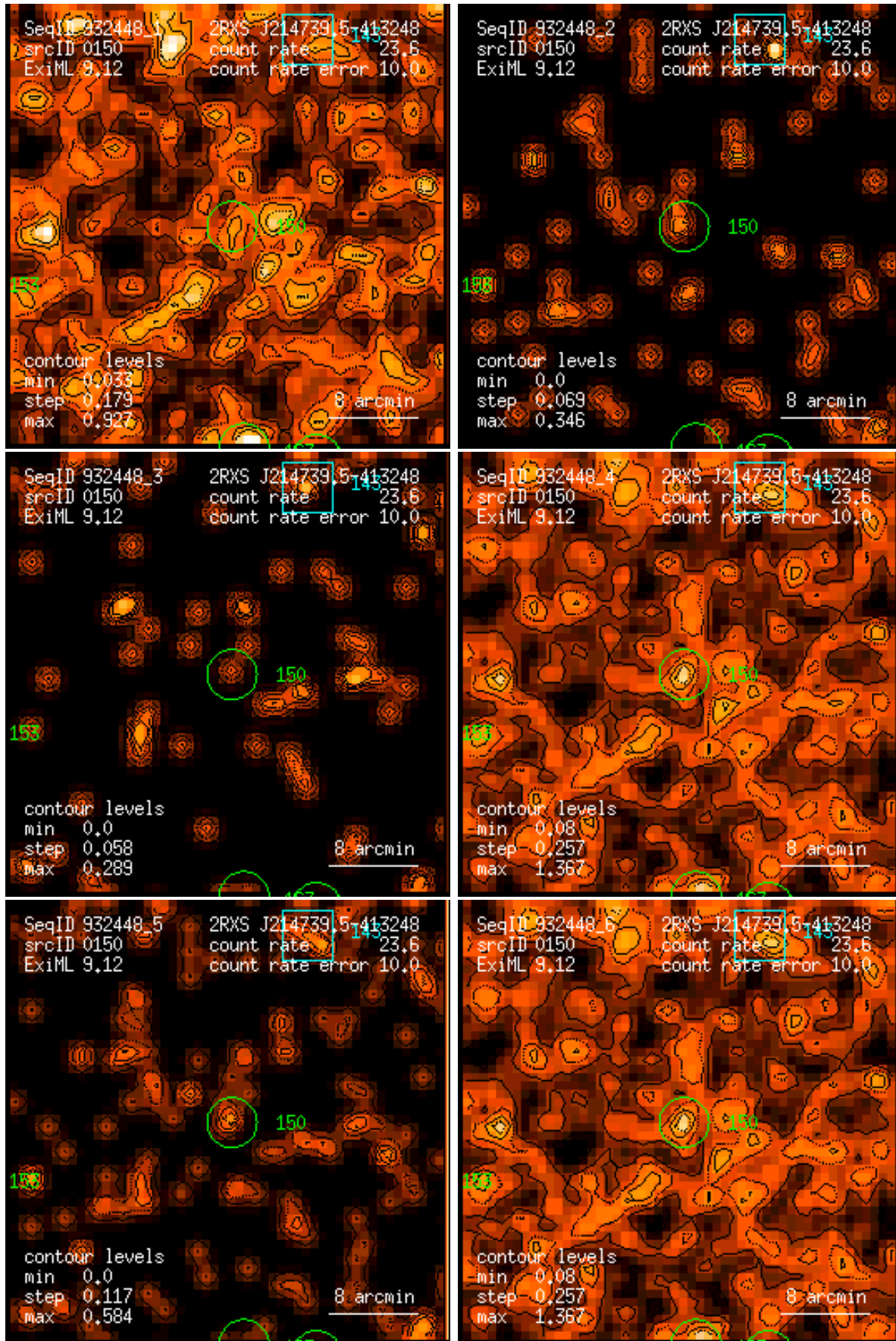
Figure 150: RASS 932448: detection 0150: band rate images, Gaussian filter: (1) PSPC channels 11 – 41, (2) 52 – 90, (3) 91 – 201, (4) 11 – 235, (5) 52 – 201, (6) 11 – 201. Broad band rates in counts/ks. Band rate contour levels in counts/ks/arcmin 2 .
