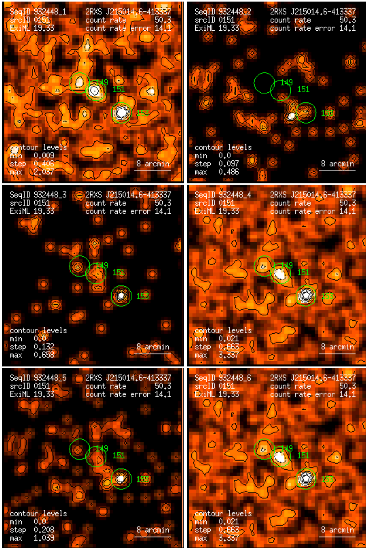
Figure 151: RASS 932448: detection 0151: band rate images, Gaussian filter: (1) PSPC channels 11 – 41, (2) 52 – 90, (3) 91 – 201, (4) 11 – 235, (5) 52 – 201, (6) 11 – 201. Broad band rates in counts/ks. Band rate contour levels in counts/ks/arcmin 2 .
