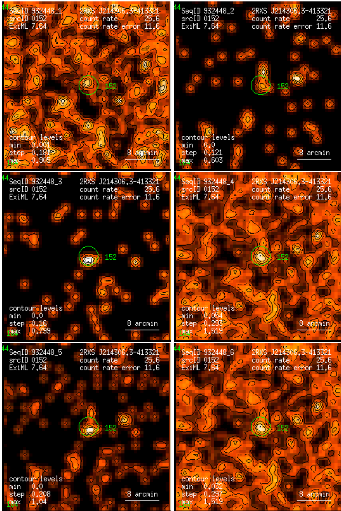
Figure 152: RASS 932448: detection 0152: band rate images, Gaussian filter: (1) PSPC channels 11 – 41, (2) 52 – 90, (3) 91 – 201, (4) 11 – 235, (5) 52 – 201, (6) 11 – 201. Broad band rates in counts/ks. Band rate contour levels in counts/ks/arcmin 2 .
