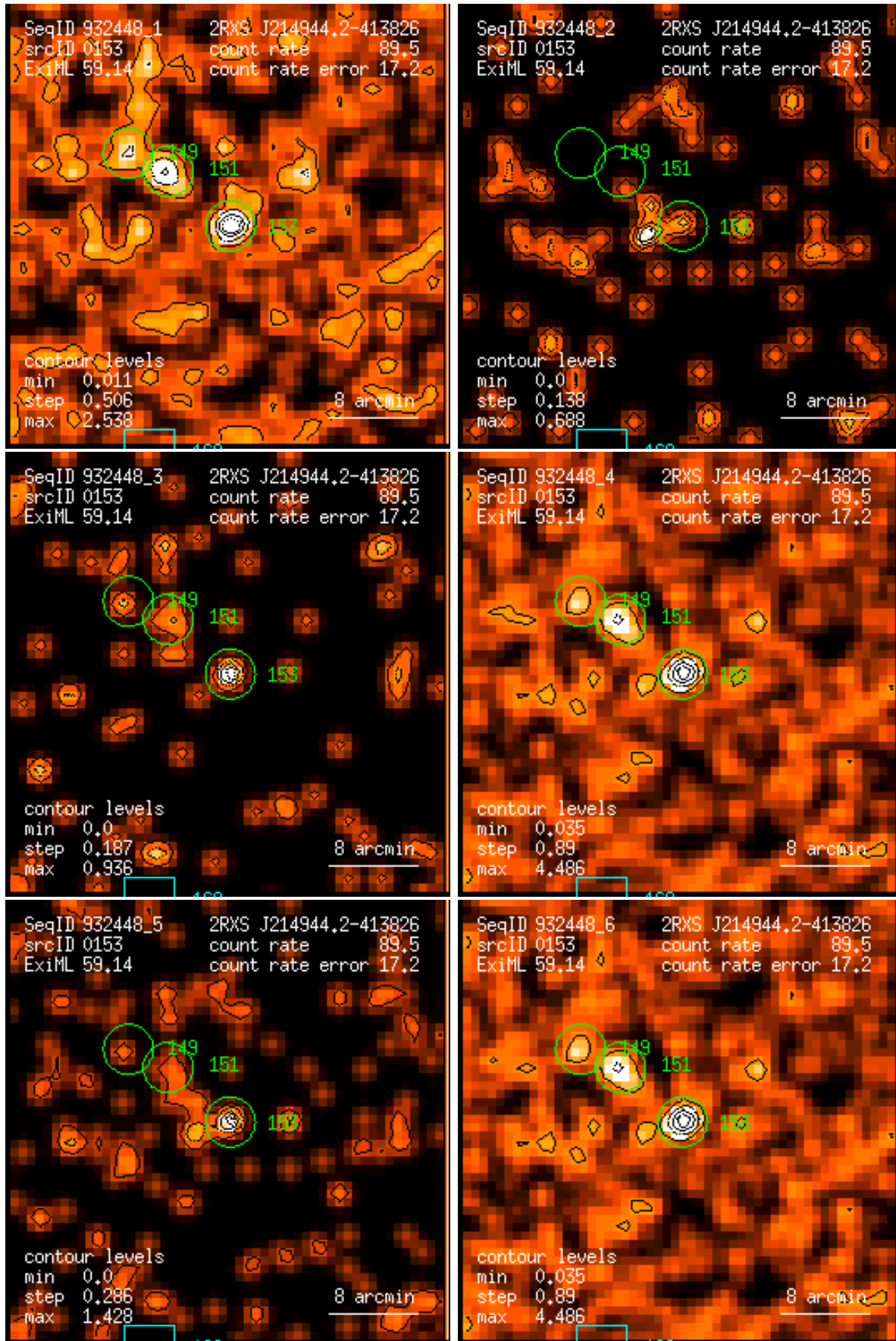
Figure 153: RASS 932448: detection 0153: band rate images, Gaussian filter: (1) PSPC channels 11 – 41, (2) 52 – 90, (3) 91 – 201, (4) 11 – 235, (5) 52 – 201, (6) 11 – 201. Broad band rates in counts/ks. Band rate contour levels in counts/ks/arcmin 2 .
