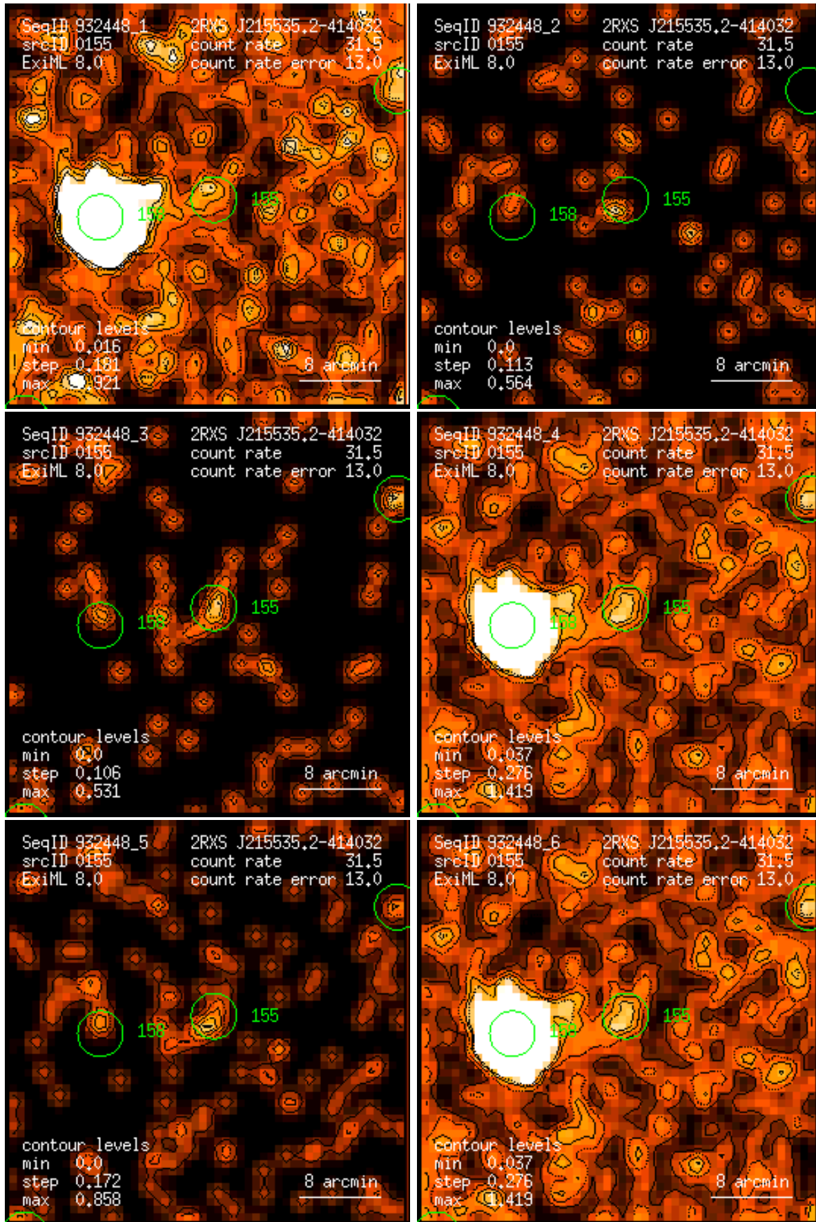
Figure 155: RASS 932448: detection 0155: band rate images, Gaussian filter: (1) PSPC channels 11 – 41, (2) 52 – 90, (3) 91 – 201, (4) 11 – 235, (5) 52 – 201, (6) 11 – 201. Broad band rates in counts/ks. Band rate contour levels in counts/ks/arcmin 2 .
