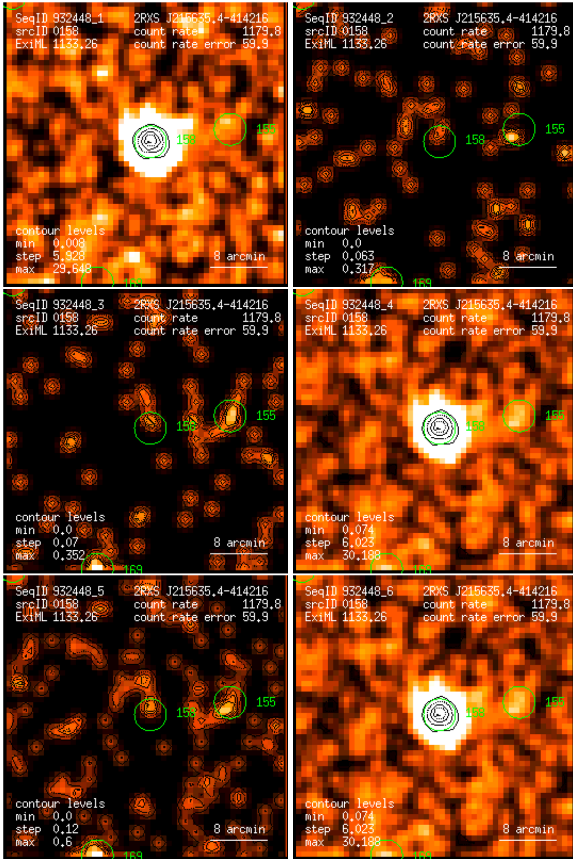
Figure 158: RASS 932448: detection 0158: band rate images, Gaussian filter: (1) PSPC channels 11 – 41, (2) 52 – 90, (3) 91 – 201, (4) 11 – 235, (5) 52 – 201, (6) 11 – 201. Broad band rates in counts/ks. Band rate contour levels in counts/ks/arcmin 2 .
