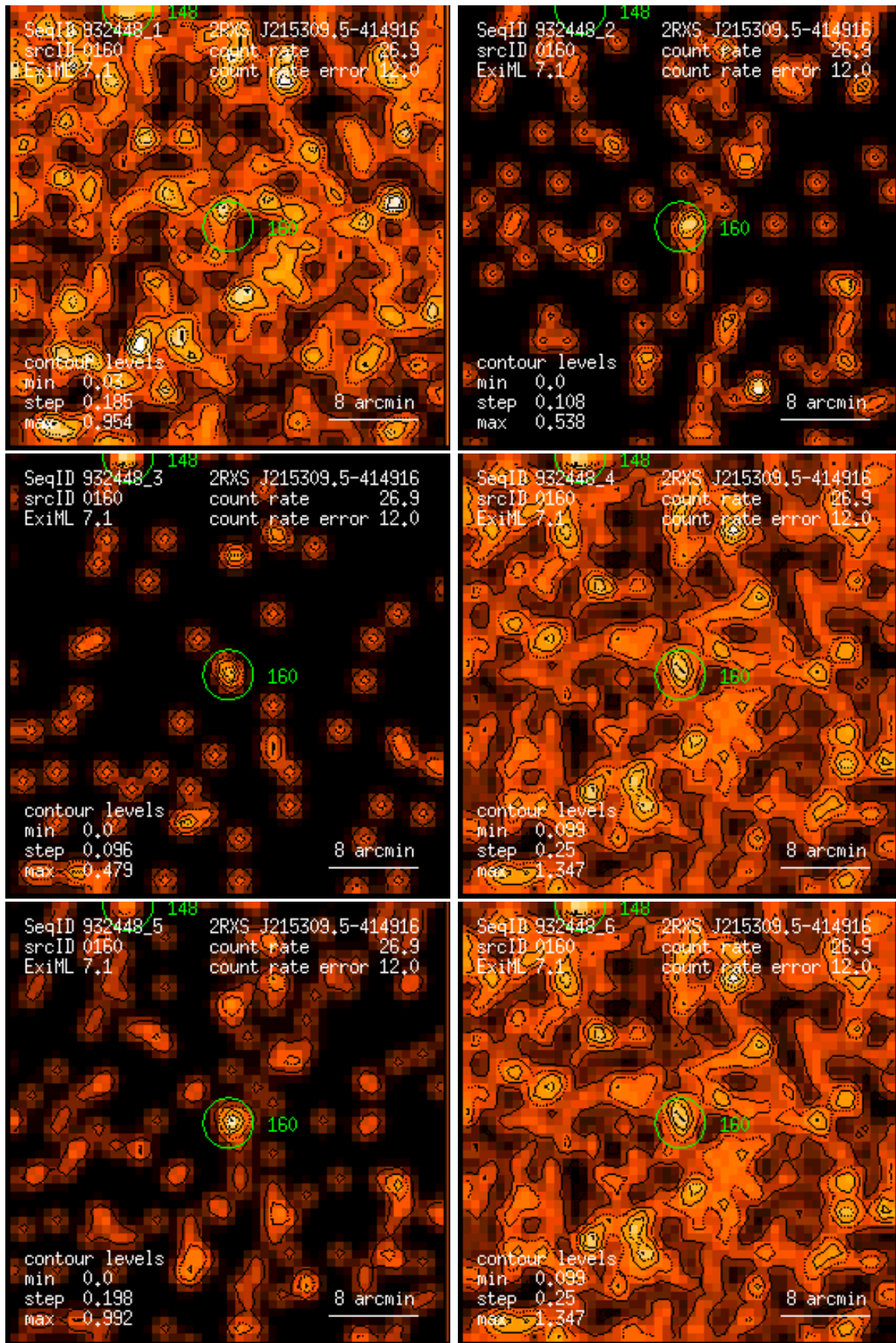
Figure 160: RASS 932448: detection 0160: band rate images, Gaussian filter: (1) PSPC channels 11 – 41, (2) 52 – 90, (3) 91 – 201, (4) 11 – 235, (5) 52 – 201, (6) 11 – 201. Broad band rates in counts/ks. Band rate contour levels in counts/ks/arcmin 2 .
