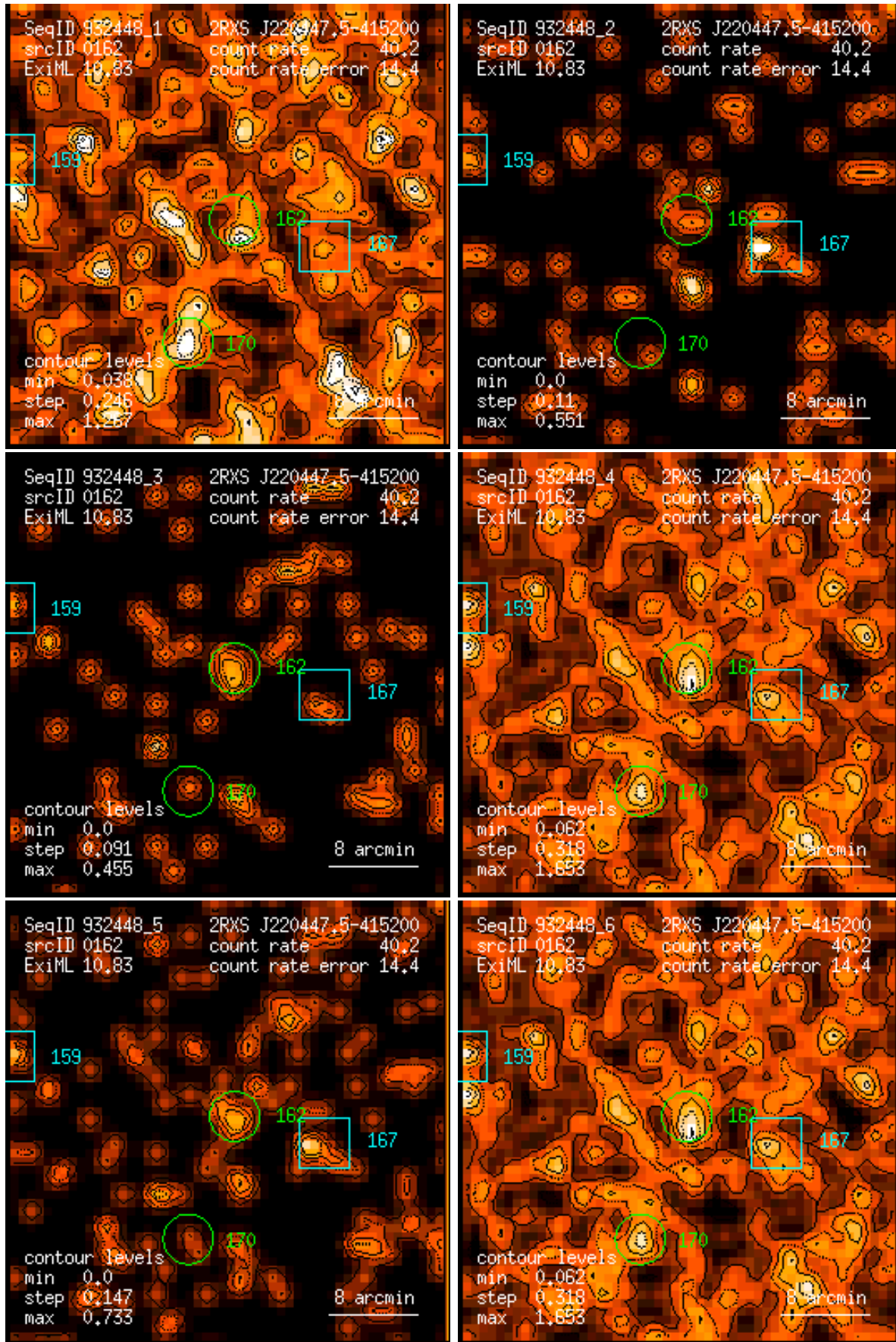
Figure 162: RASS 932448: detection 0162: band rate images, Gaussian filter: (1) PSPC channels 11 – 41, (2) 52 – 90, (3) 91 – 201, (4) 11 – 235, (5) 52 – 201, (6) 11 – 201. Broad band rates in counts/ks. Band rate contour levels in counts/ks/arcmin 2 .
