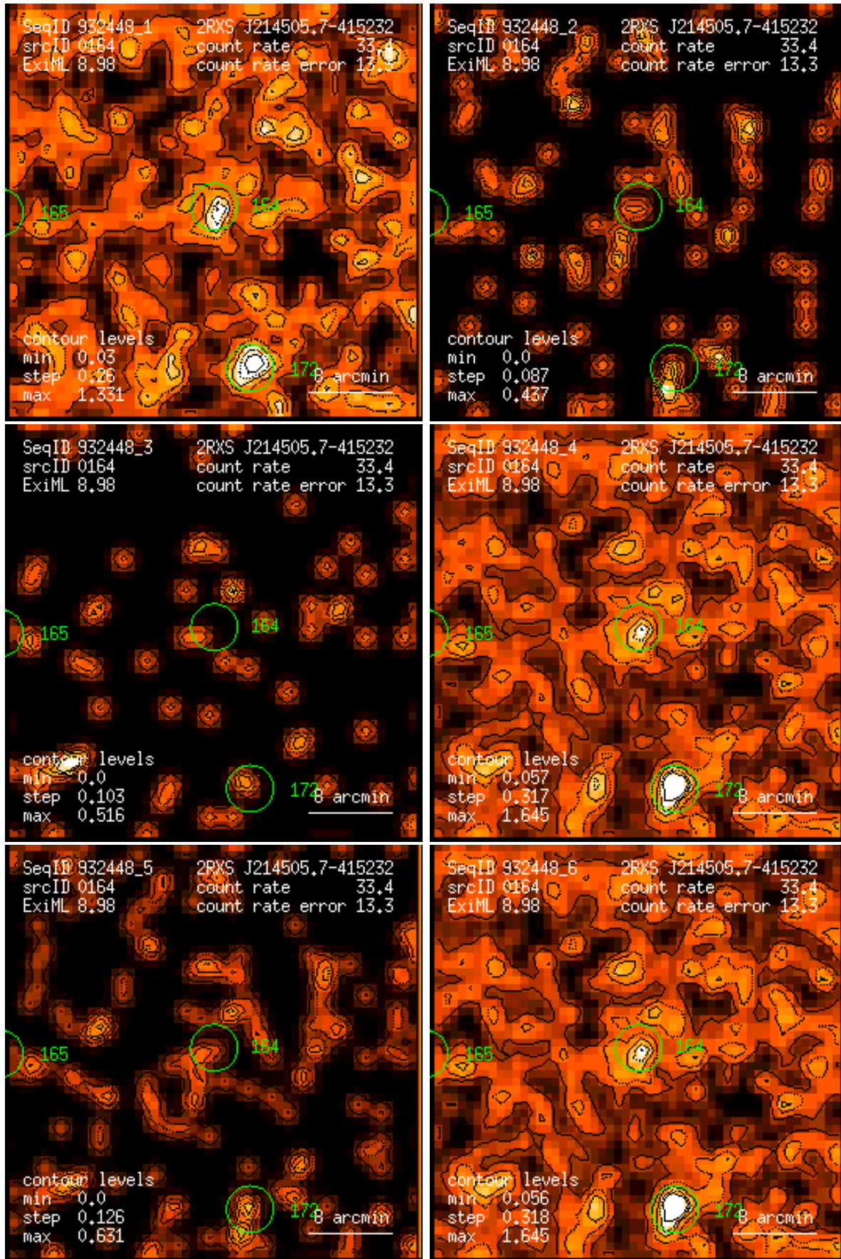
Figure 164: RASS 932448: detection 0164: band rate images, Gaussian filter: (1) PSPC channels 11 – 41, (2) 52 – 90, (3) 91 – 201, (4) 11 – 235, (5) 52 – 201, (6) 11 – 201. Broad band rates in counts/ks. Band rate contour levels in counts/ks/arcmin 2 .
