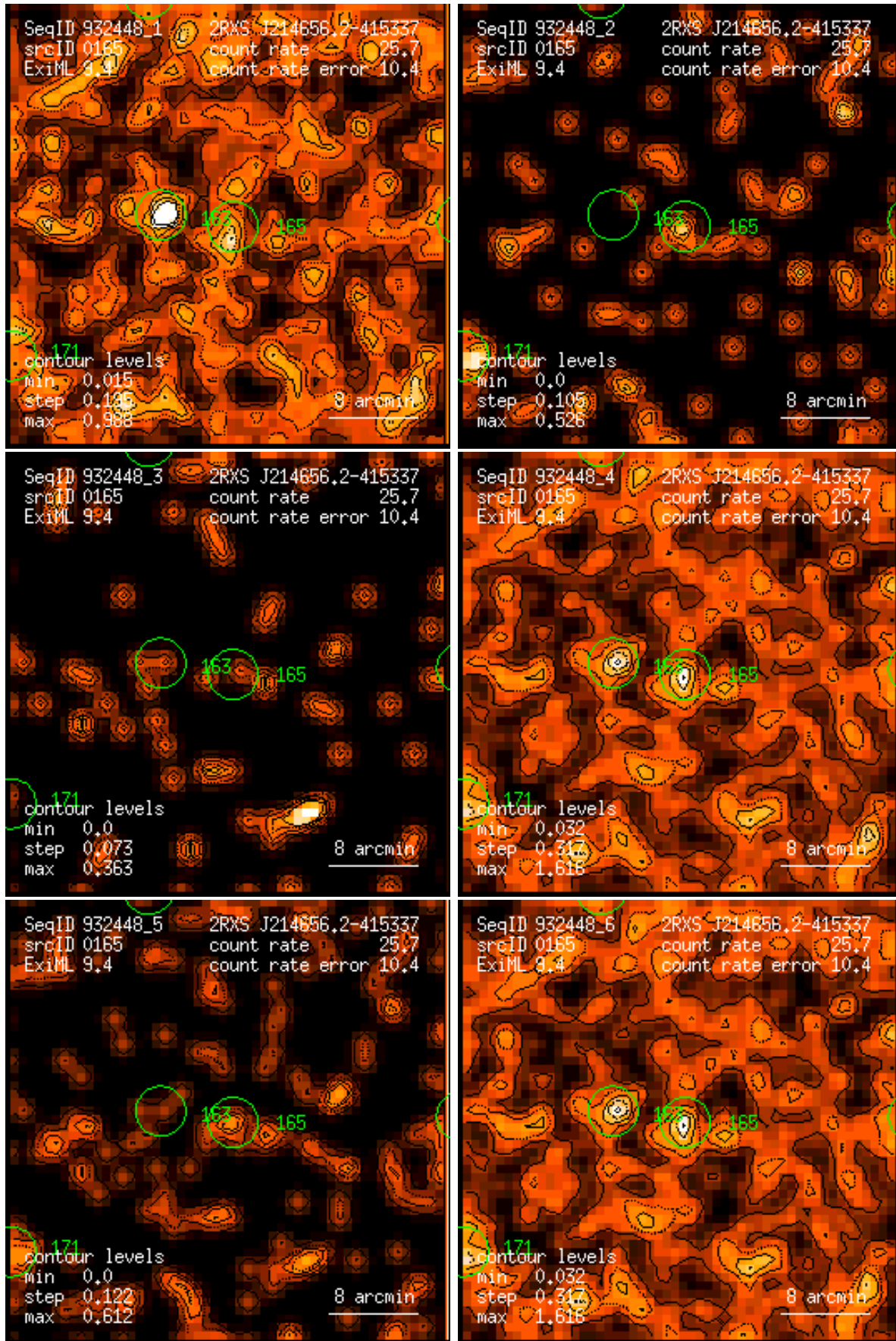
Figure 165: RASS 932448: detection 0165: band rate images, Gaussian filter: (1) PSPC channels 11 – 41, (2) 52 – 90, (3) 91 – 201, (4) 11 – 235, (5) 52 – 201, (6) 11 – 201. Broad band rates in counts/ks. Band rate contour levels in counts/ks/arcmin 2 .
