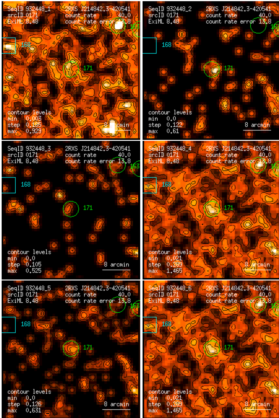
Figure 171: RASS 932448: detection 0171: band rate images, Gaussian filter: (1) PSPC channels 11 – 41, (2) 52 – 90, (3) 91 – 201, (4) 11 – 235, (5) 52 – 201, (6) 11 – 201. Broad band rates in counts/ks. Band rate contour levels in counts/ks/arcmin 2 .
