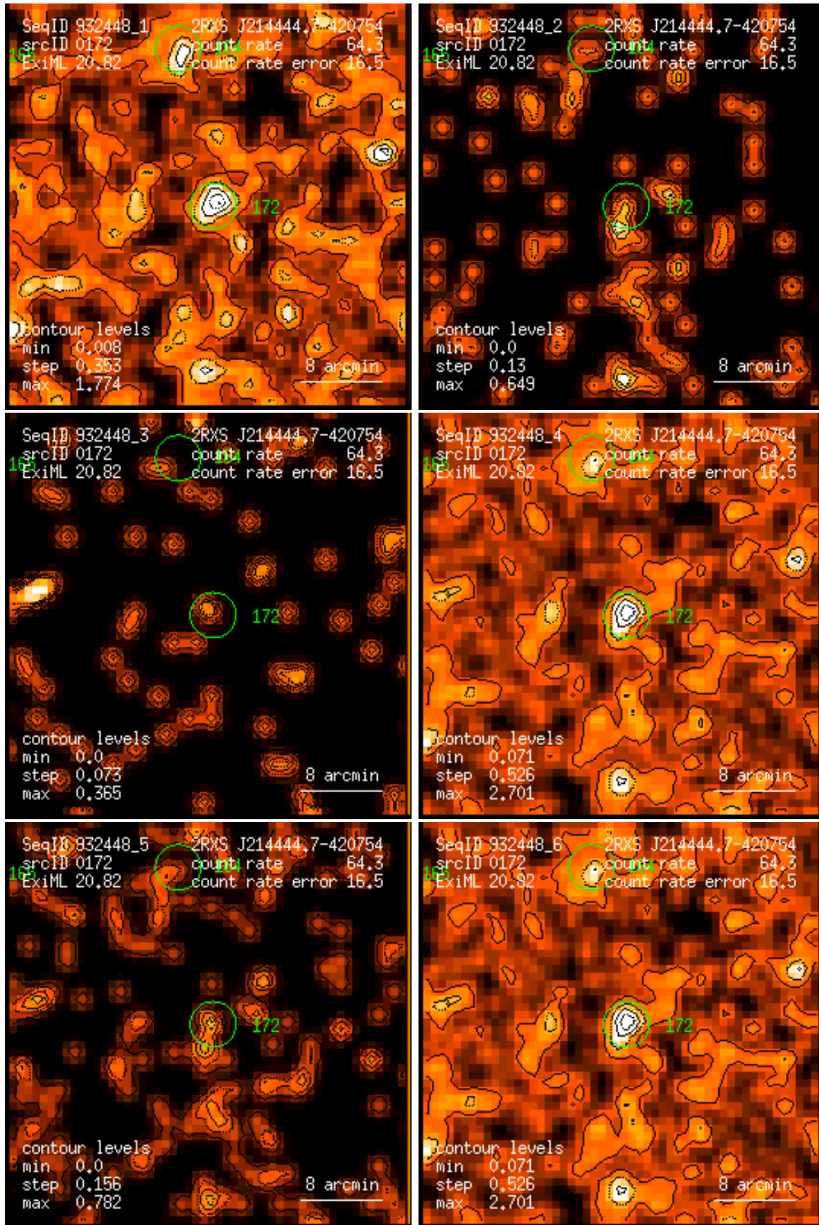
Figure 172: RASS 932448: detection 0172: band rate images, Gaussian filter: (1) PSPC channels 11 – 41, (2) 52 – 90, (3) 91 – 201, (4) 11 – 235, (5) 52 – 201, (6) 11 – 201. Broad band rates in counts/ks. Band rate contour levels in counts/ks/arcmin 2 .
