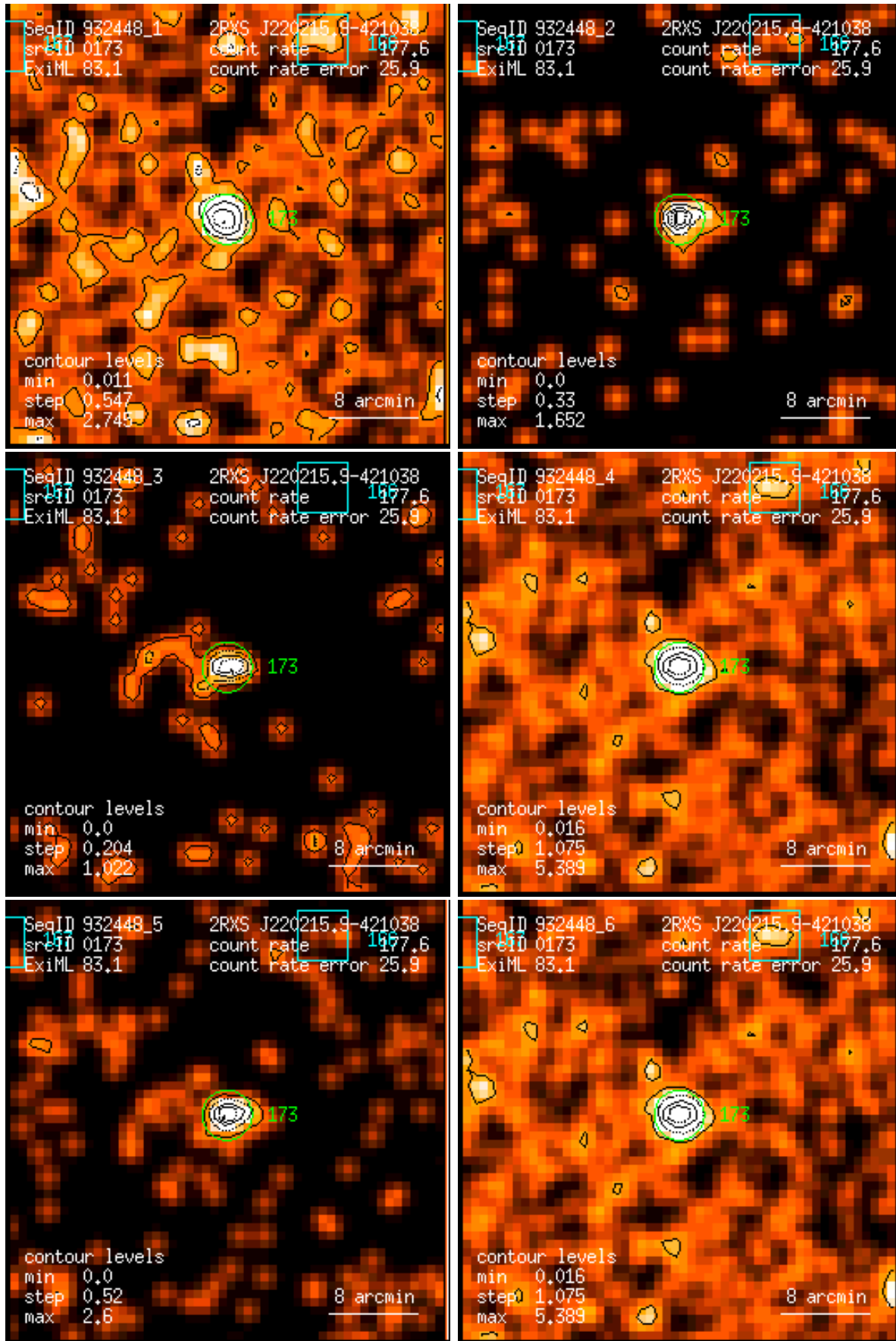
Figure 173: RASS 932448: detection 0173: band rate images, Gaussian filter: (1) PSPC channels 11 – 41, (2) 52 – 90, (3) 91 – 201, (4) 11 – 235, (5) 52 – 201, (6) 11 – 201. Broad band rates in counts/ks. Band rate contour levels in counts/ks/arcmin 2 .
