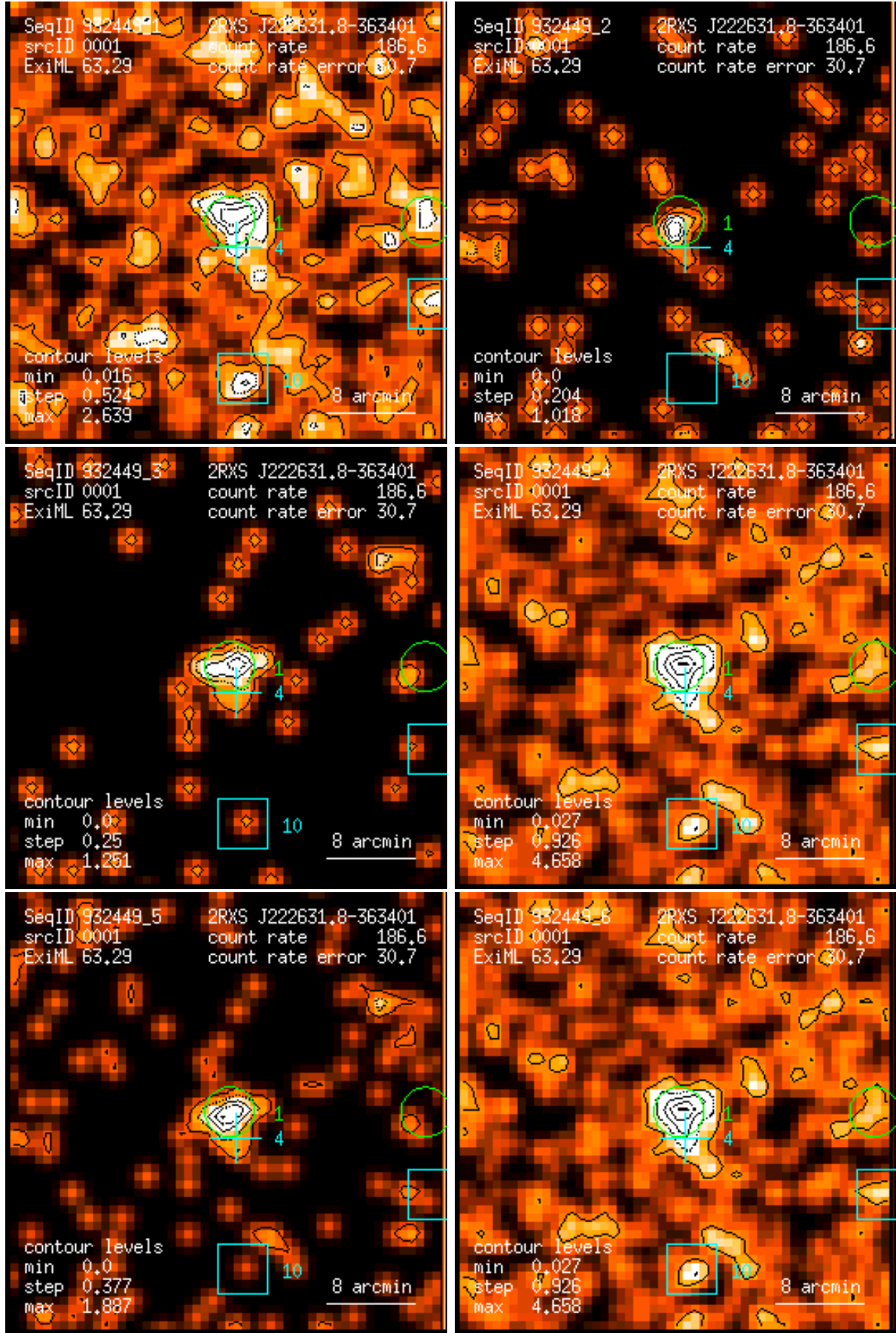
Figure 1: RASS 932449: detection 0001: band rate images, Gaussian filter: (1) PSPC channels 11 – 41, (2) 52 – 90, (3) 91 – 201, (4) 11 – 235, (5) 52 – 201, (6) 11 – 201. Broad band rates in counts/ks. Band rate contour levels in counts/ks/arcmin 2 .
