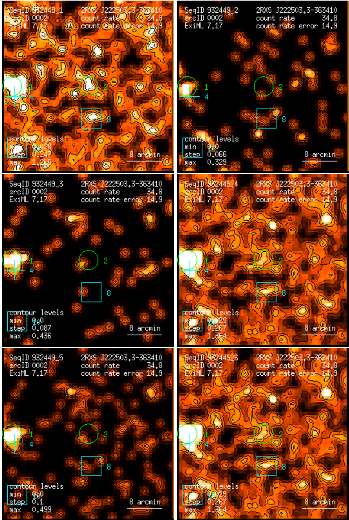
Figure 2: RASS 932449: detection 0002: band rate images, Gaussian filter: (1) PSPC channels 11 – 41, (2) 52 – 90, (3) 91 – 201, (4) 11 – 235, (5) 52 – 201, (6) 11 – 201. Broad band rates in counts/ks. Band rate contour levels in counts/ks/arcmin 2 .
