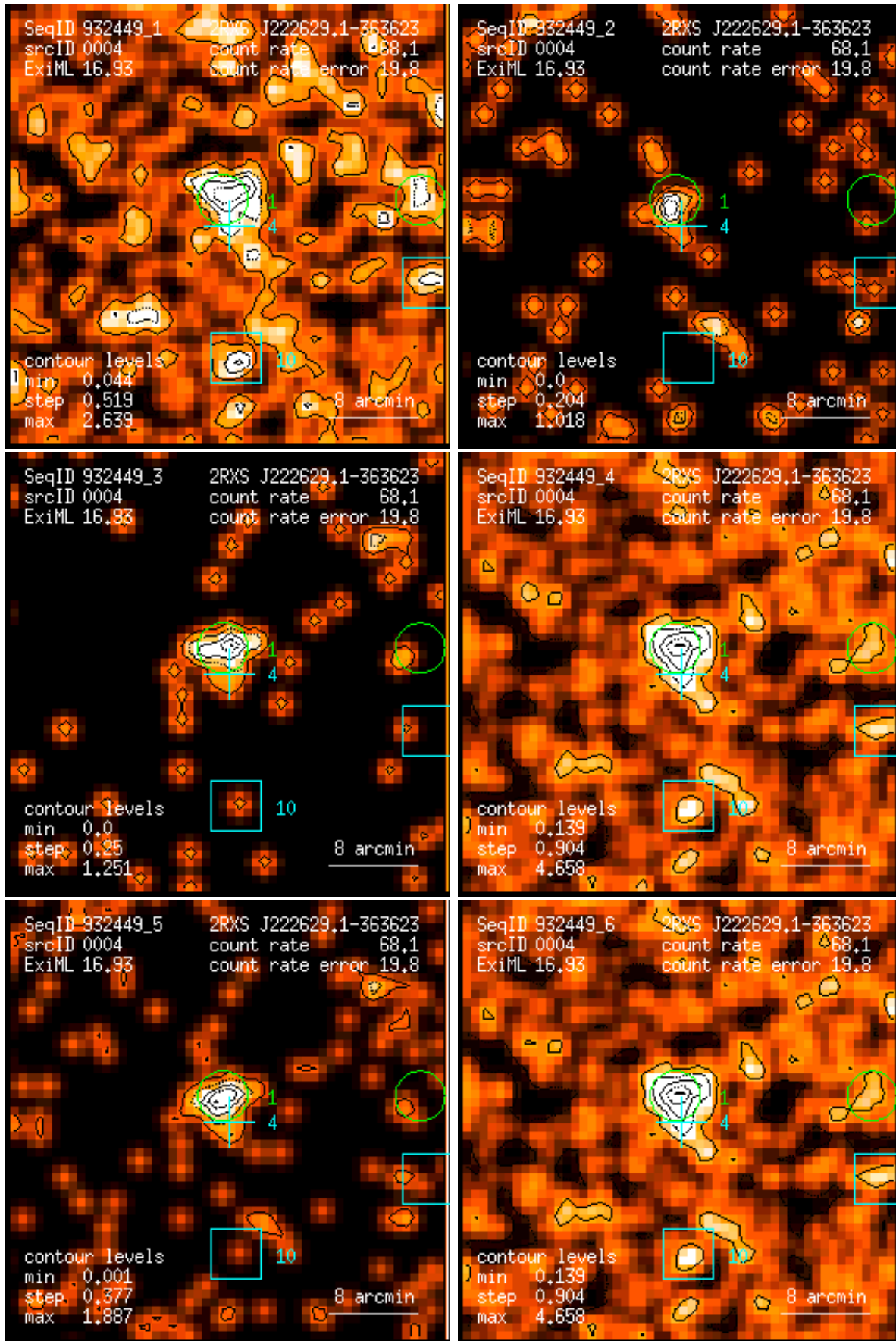
Figure 4: RASS 932449: detection 0004: band rate images, Gaussian filter: (1) PSPC channels 11 – 41, (2) 52 – 90, (3) 91 – 201, (4) 11 – 235, (5) 52 – 201, (6) 11 – 201. Broad band rates in counts/ks. Band rate contour levels in counts/ks/arcmin 2 .
