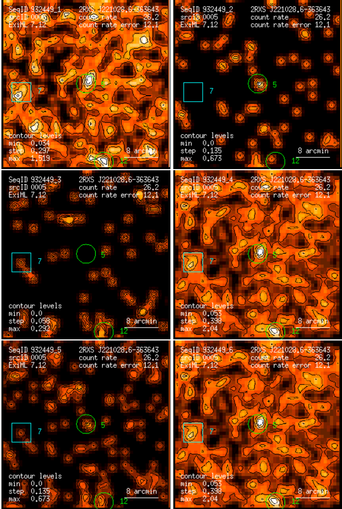
Figure 5: RASS 932449: detection 0005: band rate images, Gaussian filter: (1) PSPC channels 11 – 41, (2) 52 – 90, (3) 91 – 201, (4) 11 – 235, (5) 52 – 201, (6) 11 – 201. Broad band rates in counts/ks. Band rate contour levels in counts/ks/arcmin 2 .
