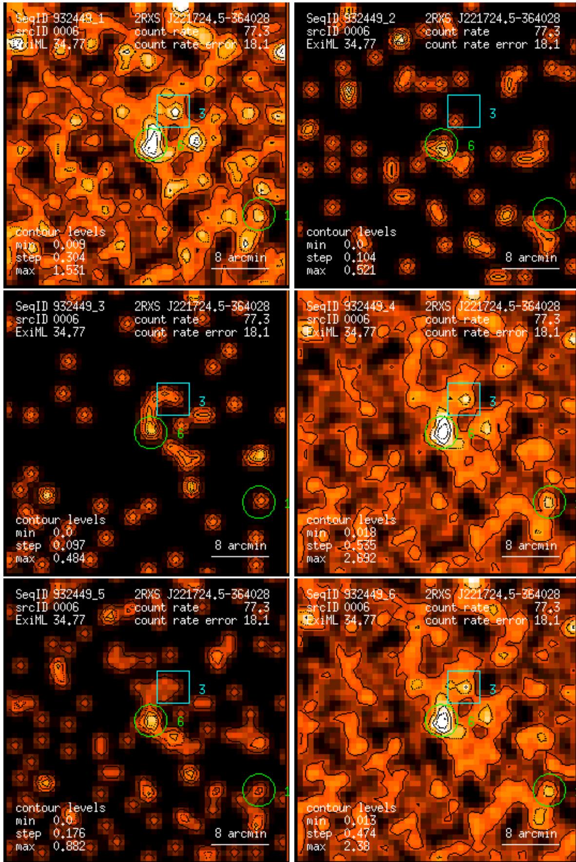
Figure 6: RASS 932449: detection 0006: band rate images, Gaussian filter: (1) PSPC channels 11 – 41, (2) 52 – 90, (3) 91 – 201, (4) 11 – 235, (5) 52 – 201, (6) 11 – 201. Broad band rates in counts/ks. Band rate contour levels in counts/ks/arcmin 2 .
